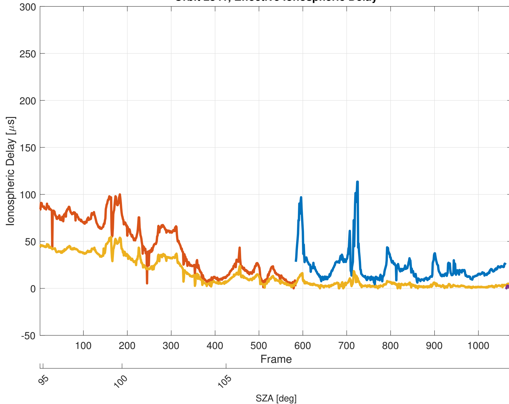
Orbit 2841, Effective Ionospheric Delay
