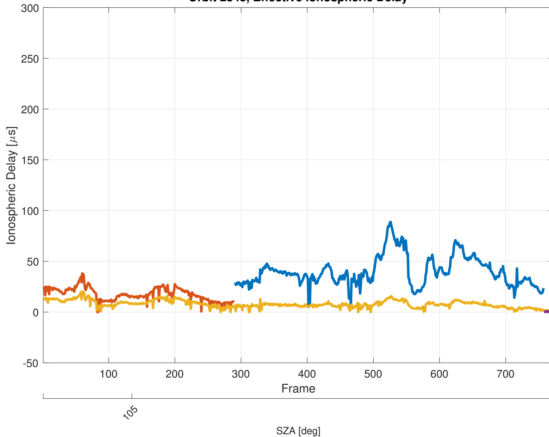
Orbit 2843, Effective Ionospheric Delay
