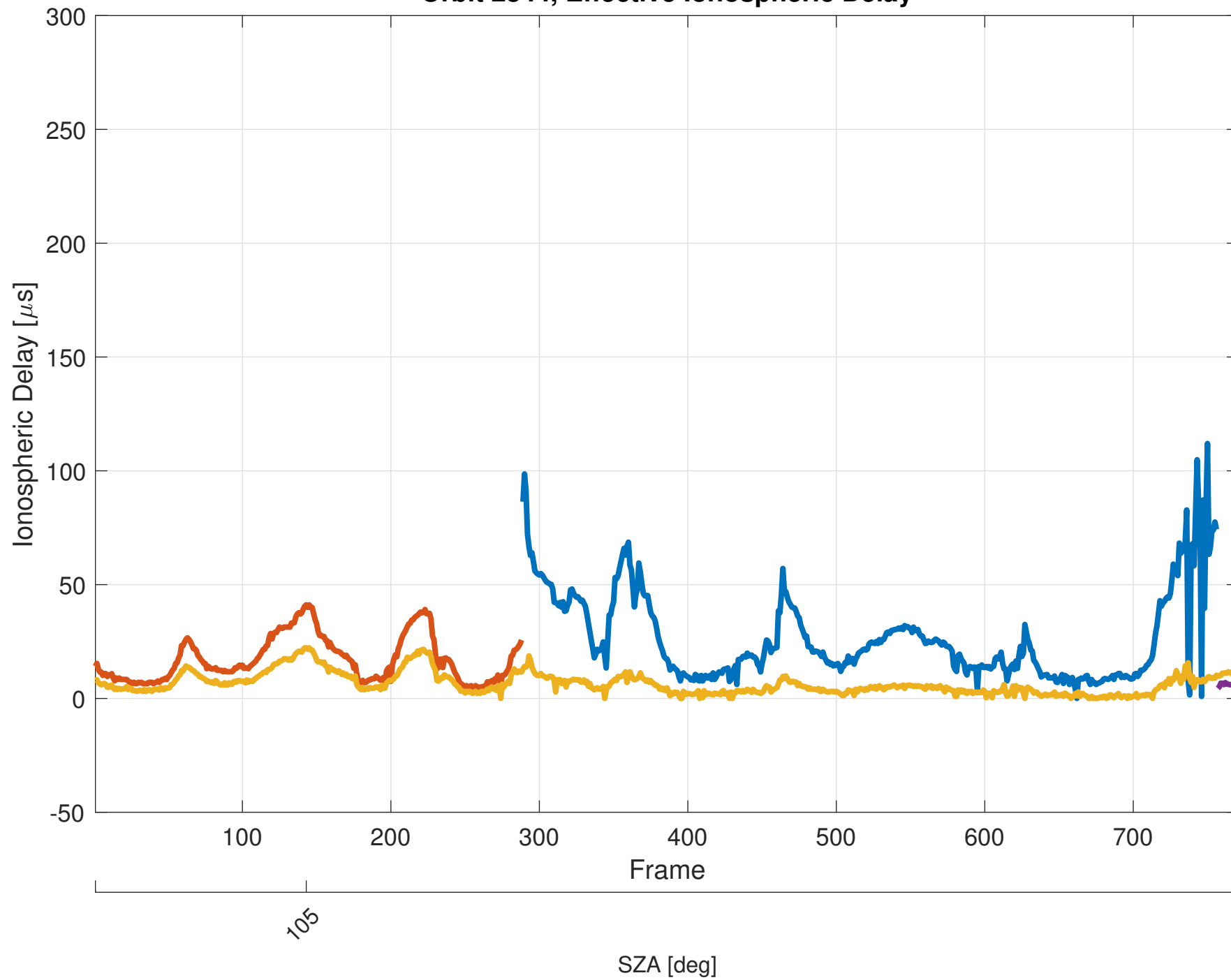
Orbit 2844, Effective Ionospheric Delay
