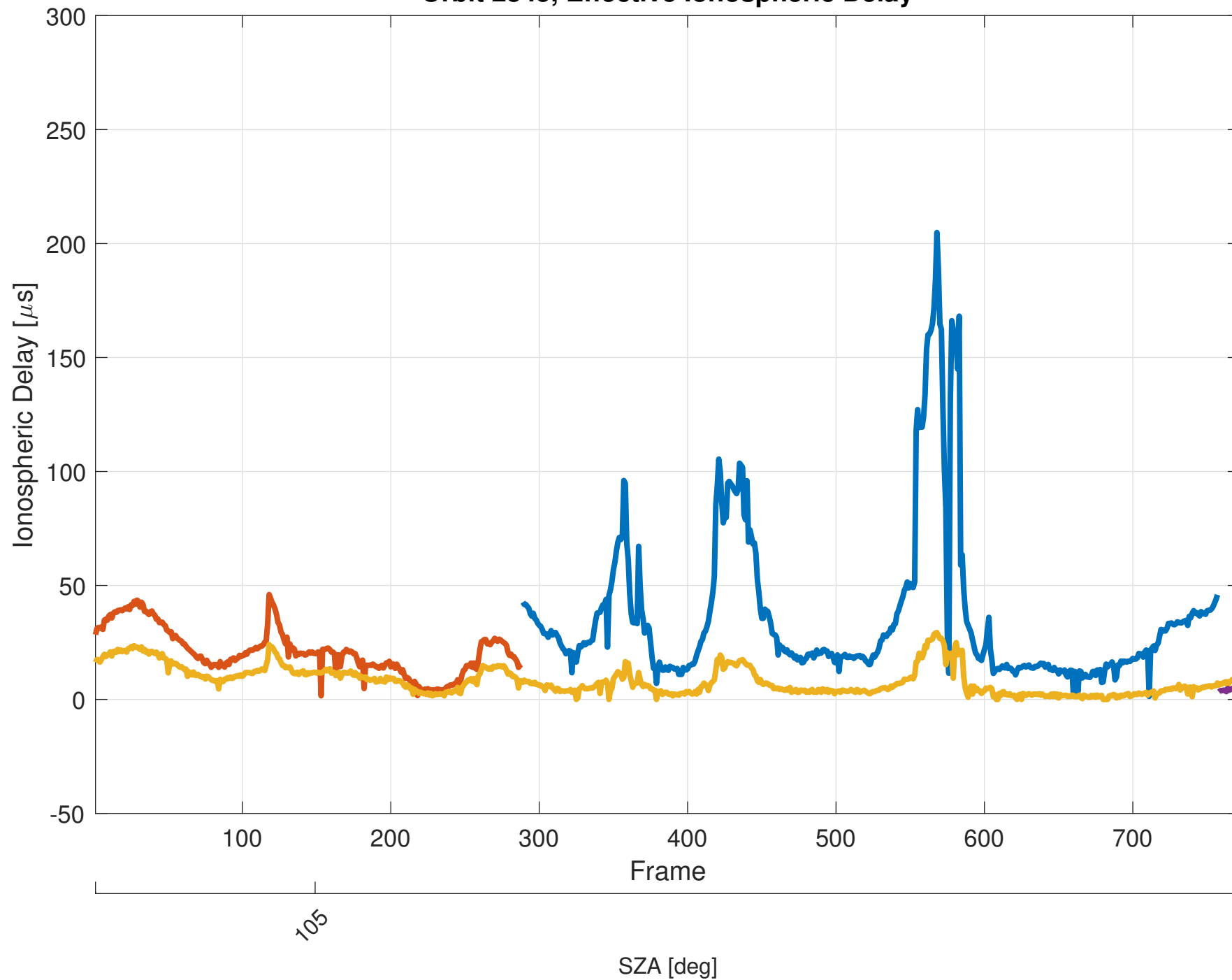
Orbit 2845, Effective Ionospheric Delay
