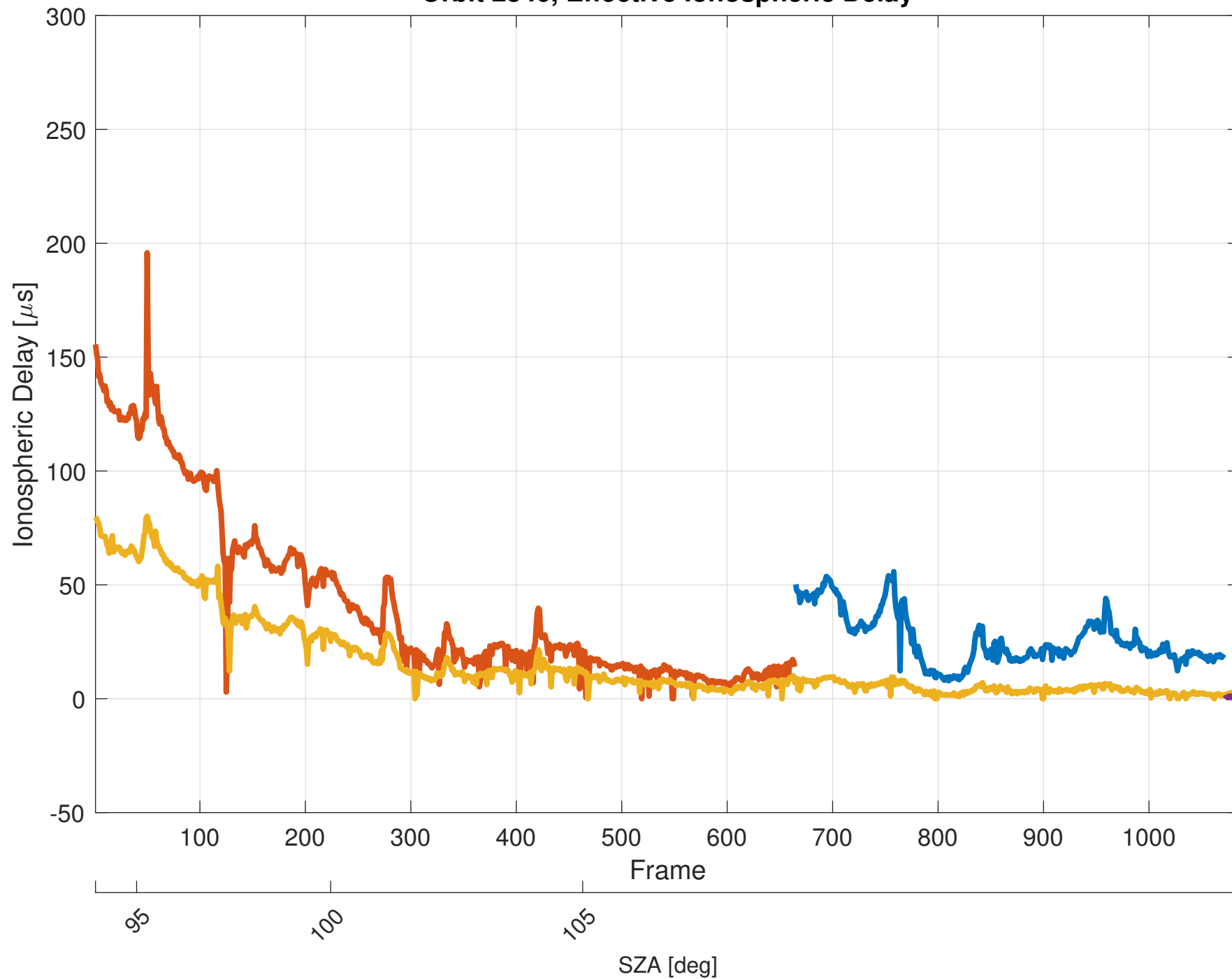
Orbit 2846, Effective Ionospheric Delay
