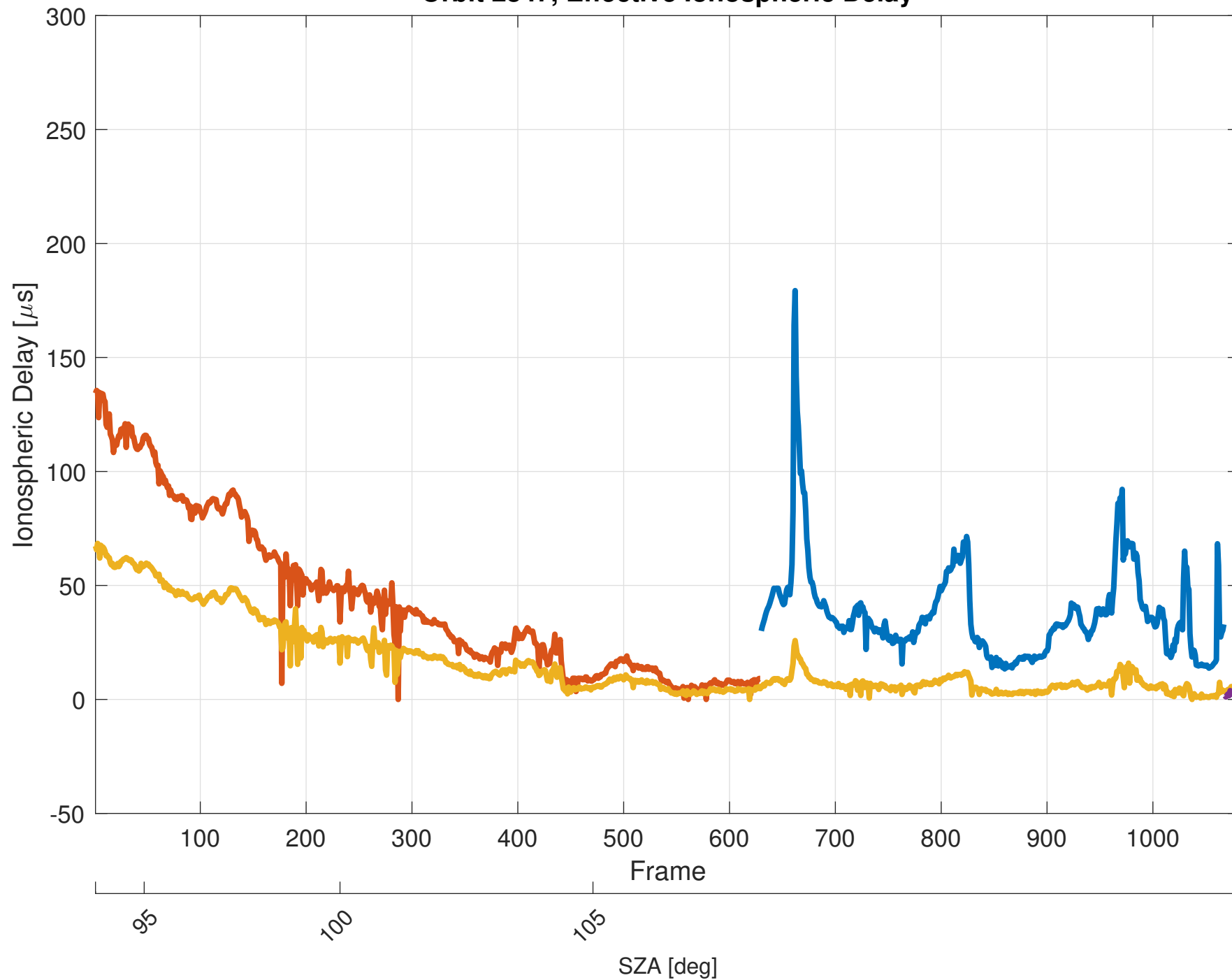
Orbit 2847, Effective Ionospheric Delay
