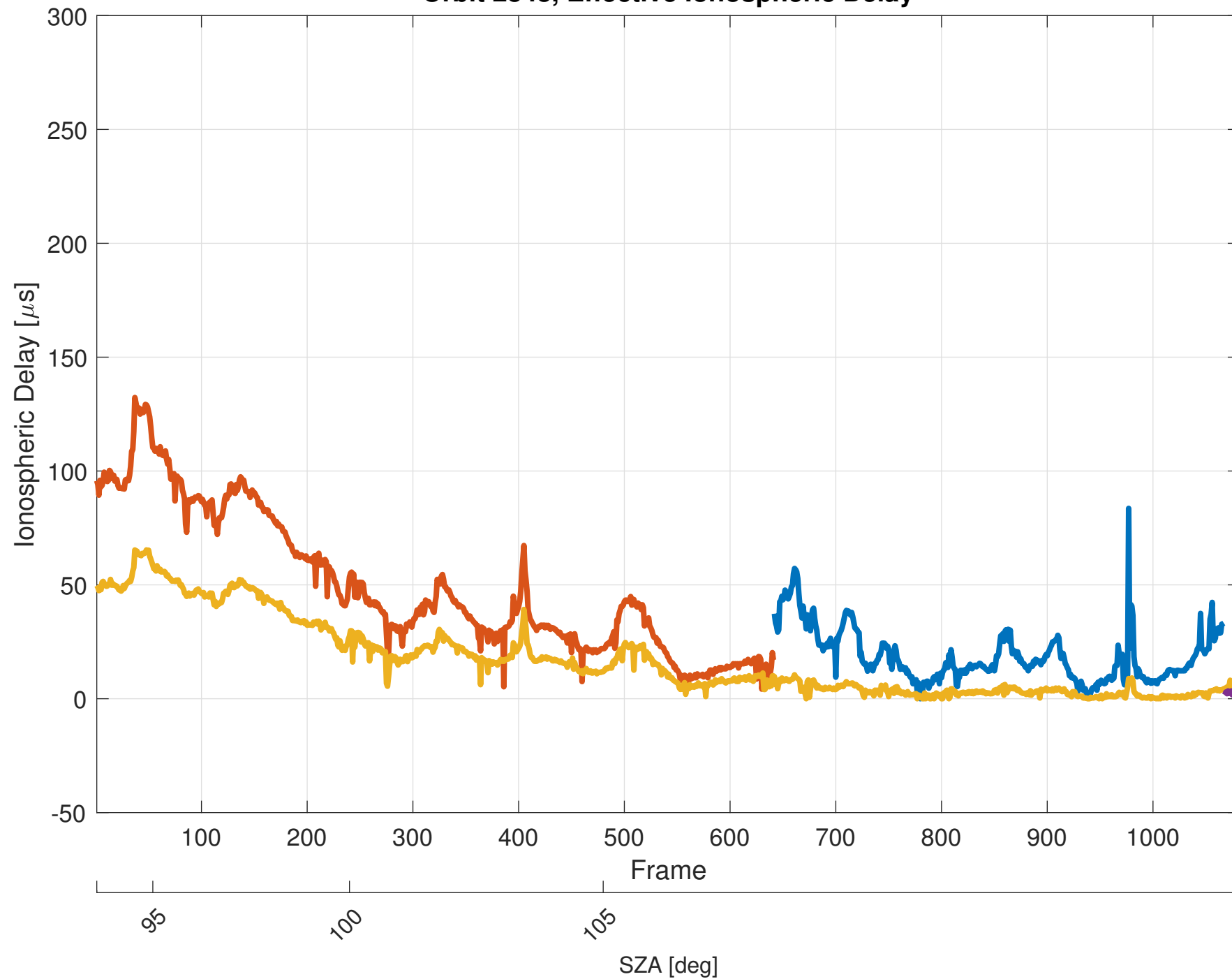
Orbit 2848, Effective Ionospheric Delay
