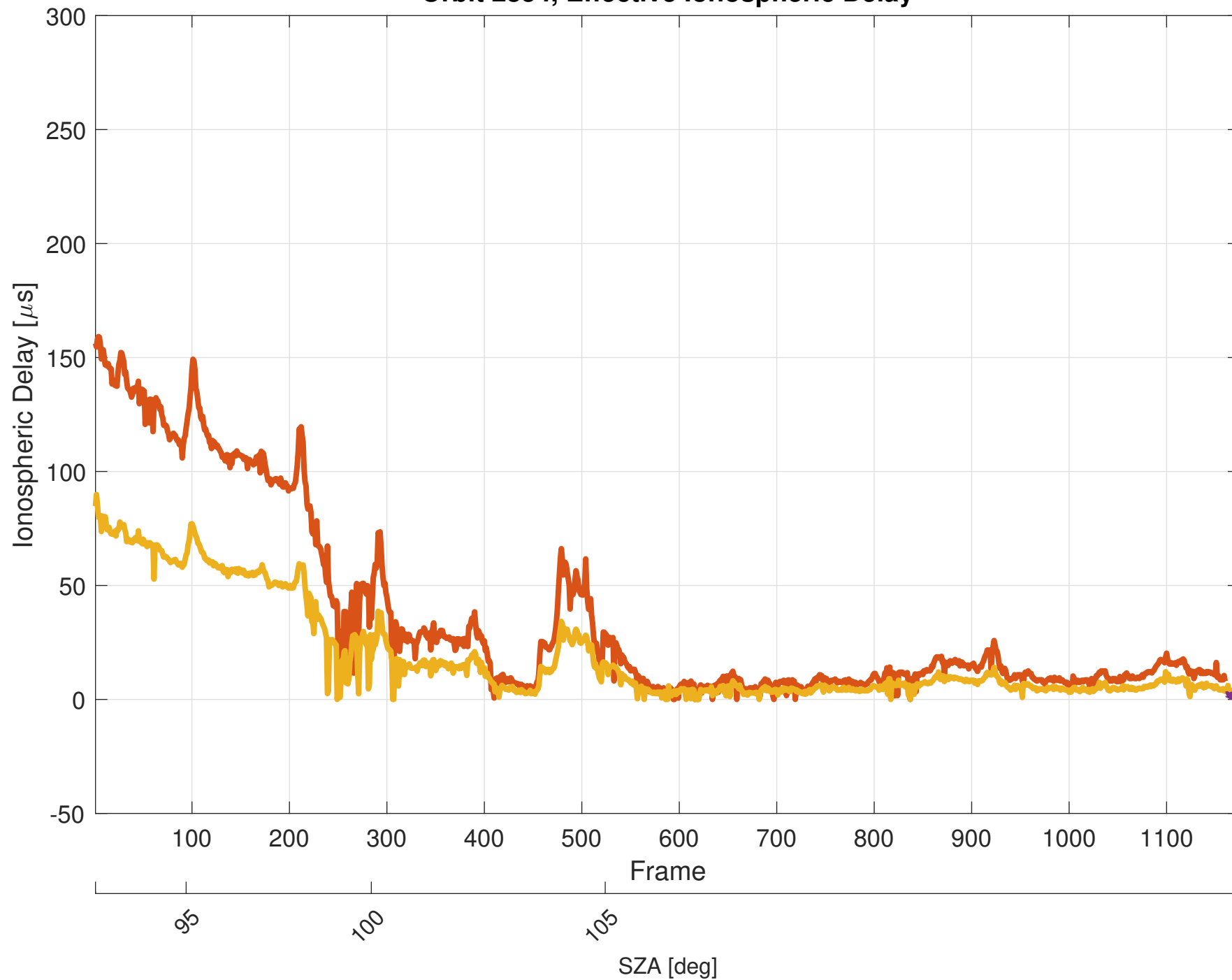
Orbit 2854, Effective Ionospheric Delay
