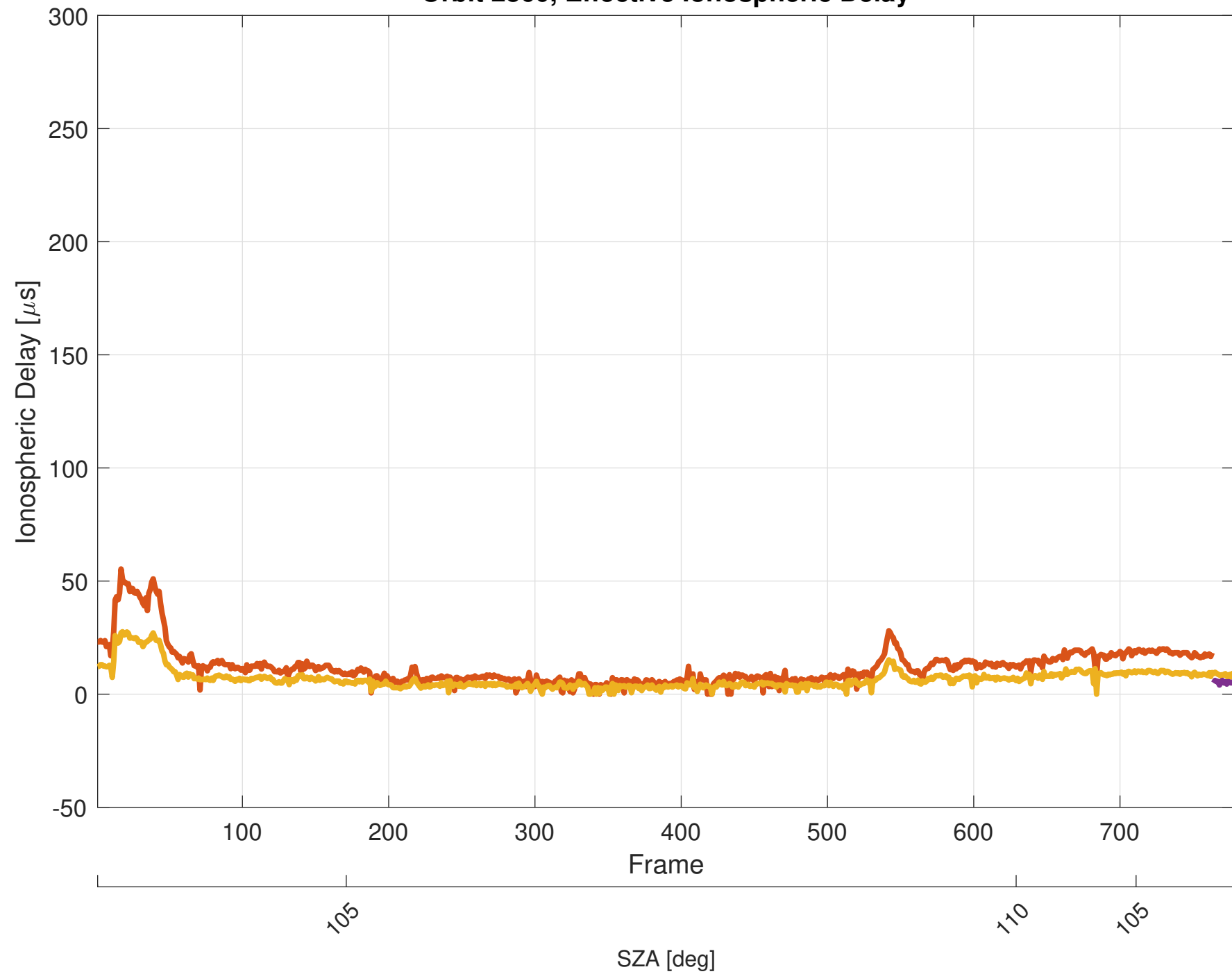
Orbit 2860, Effective Ionospheric Delay
