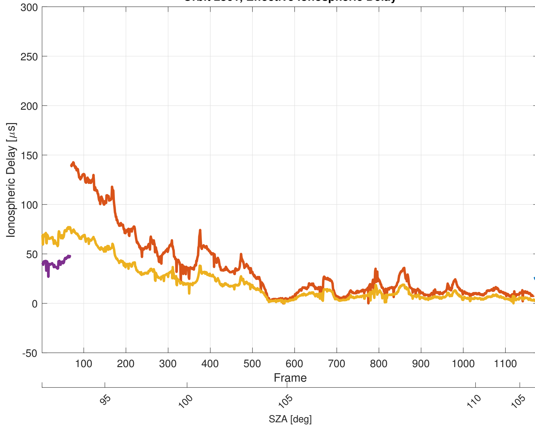
Orbit 2861, Effective Ionospheric Delay
