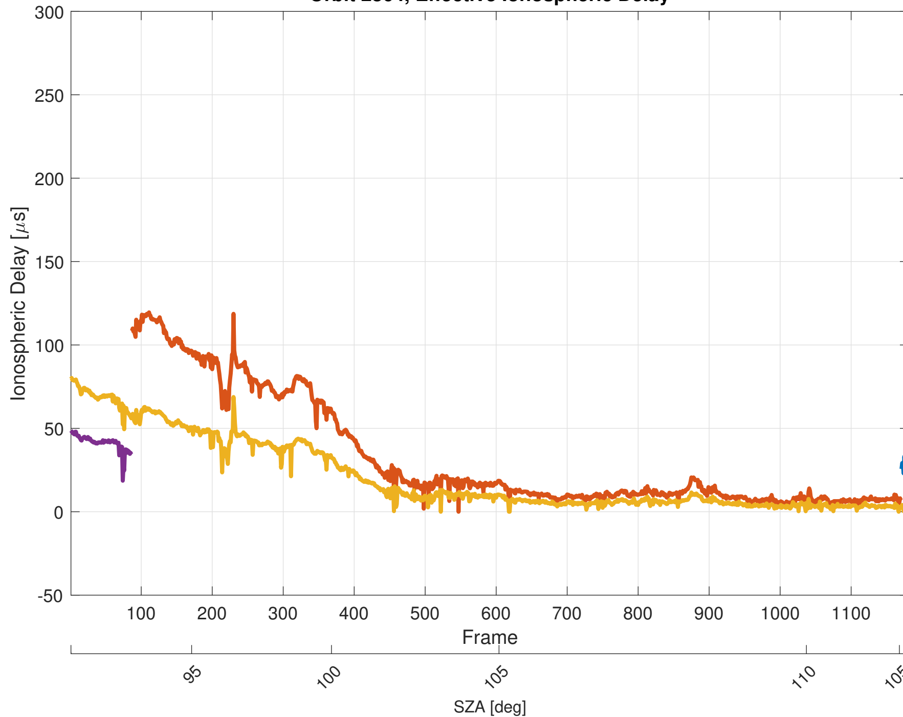
Orbit 2864, Effective Ionospheric Delay
