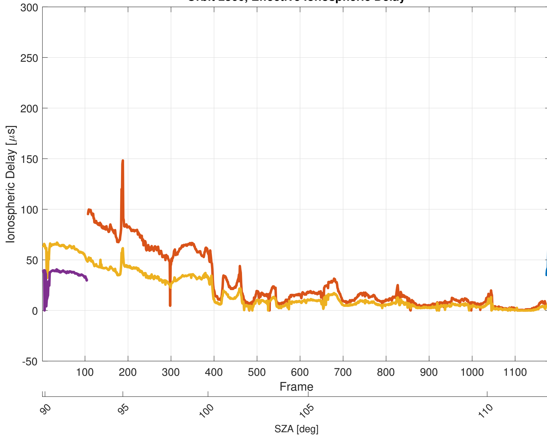
Orbit 2866, Effective Ionospheric Delay
