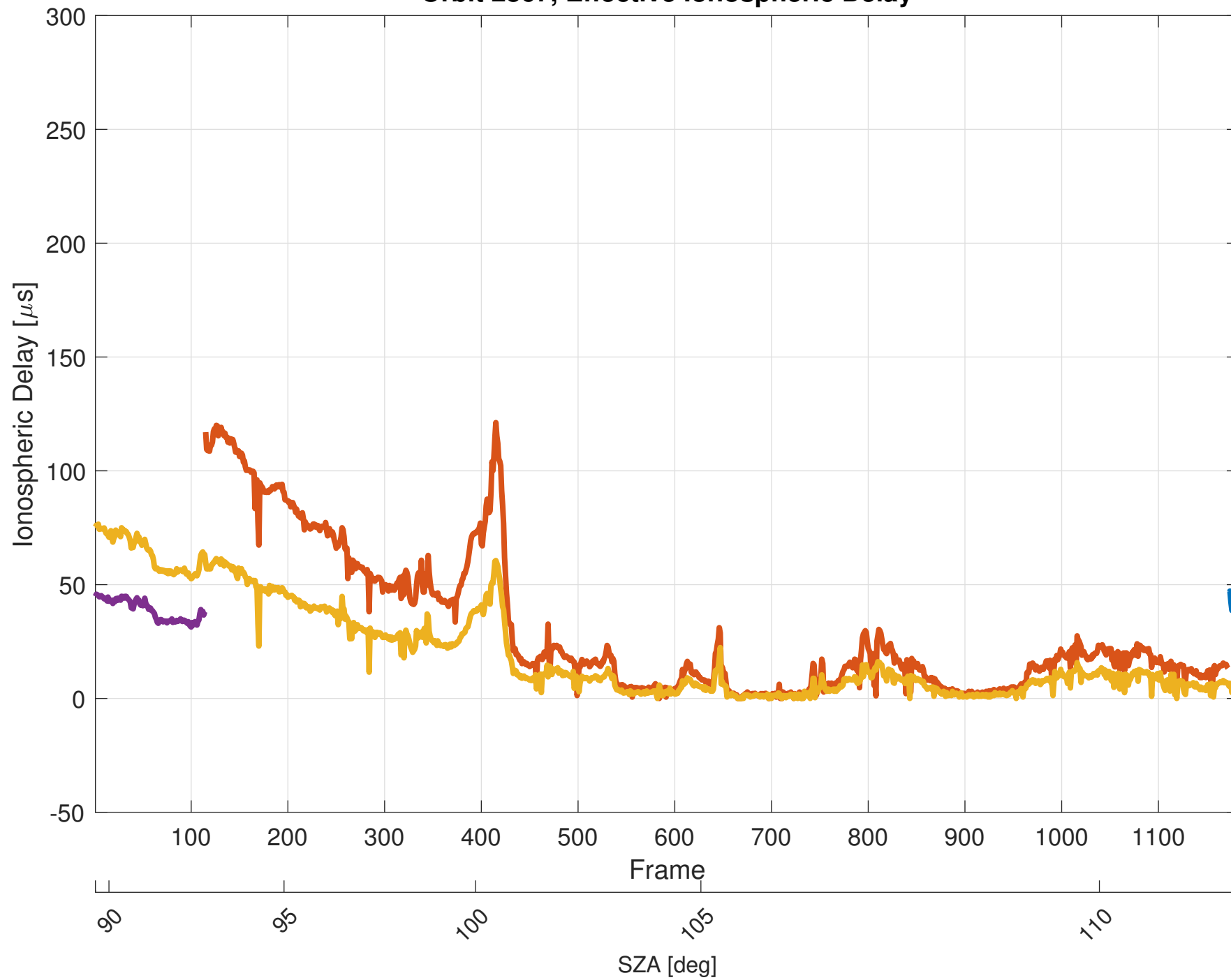
Orbit 2867, Effective Ionospheric Delay
