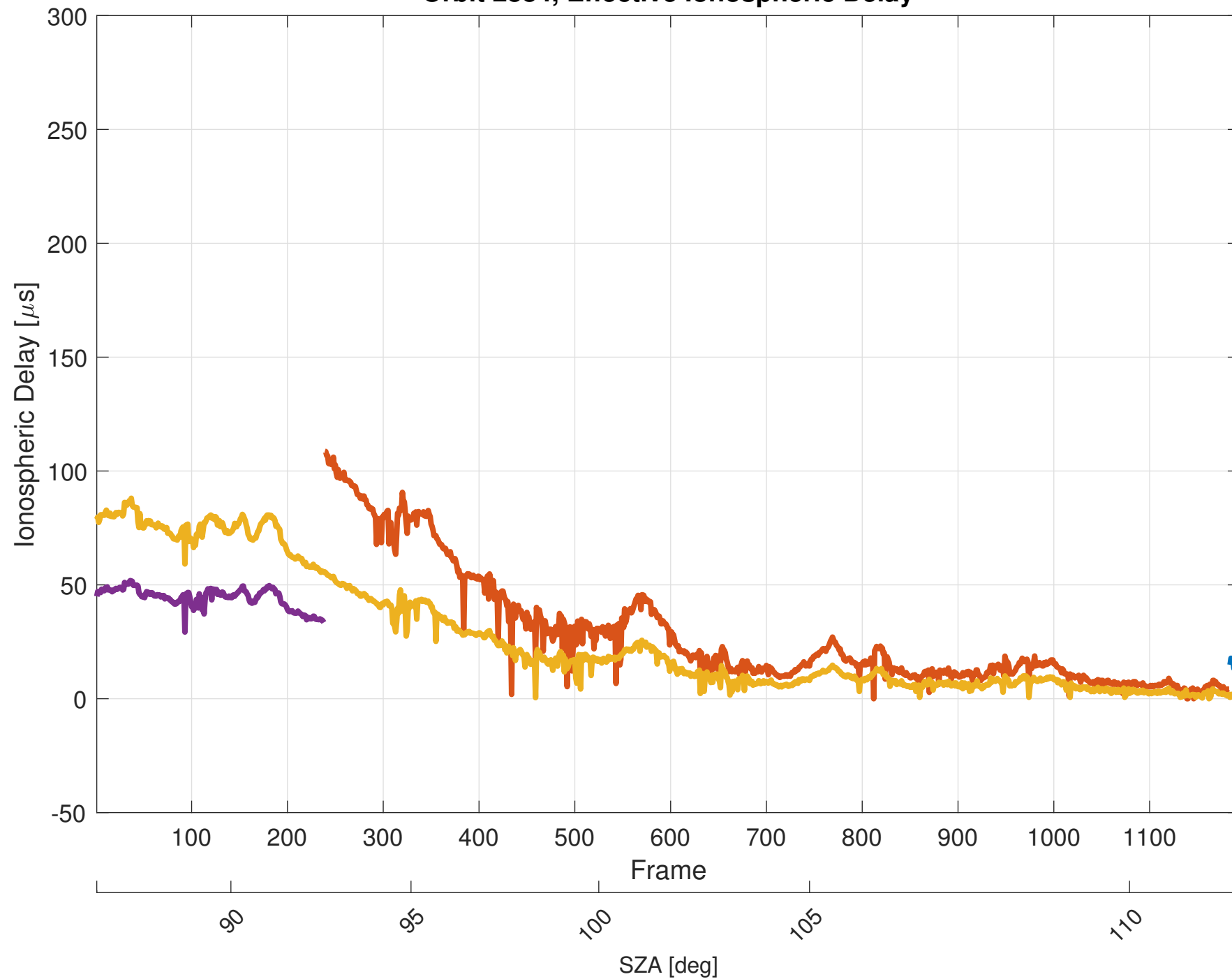
Orbit 2884, Effective Ionospheric Delay
