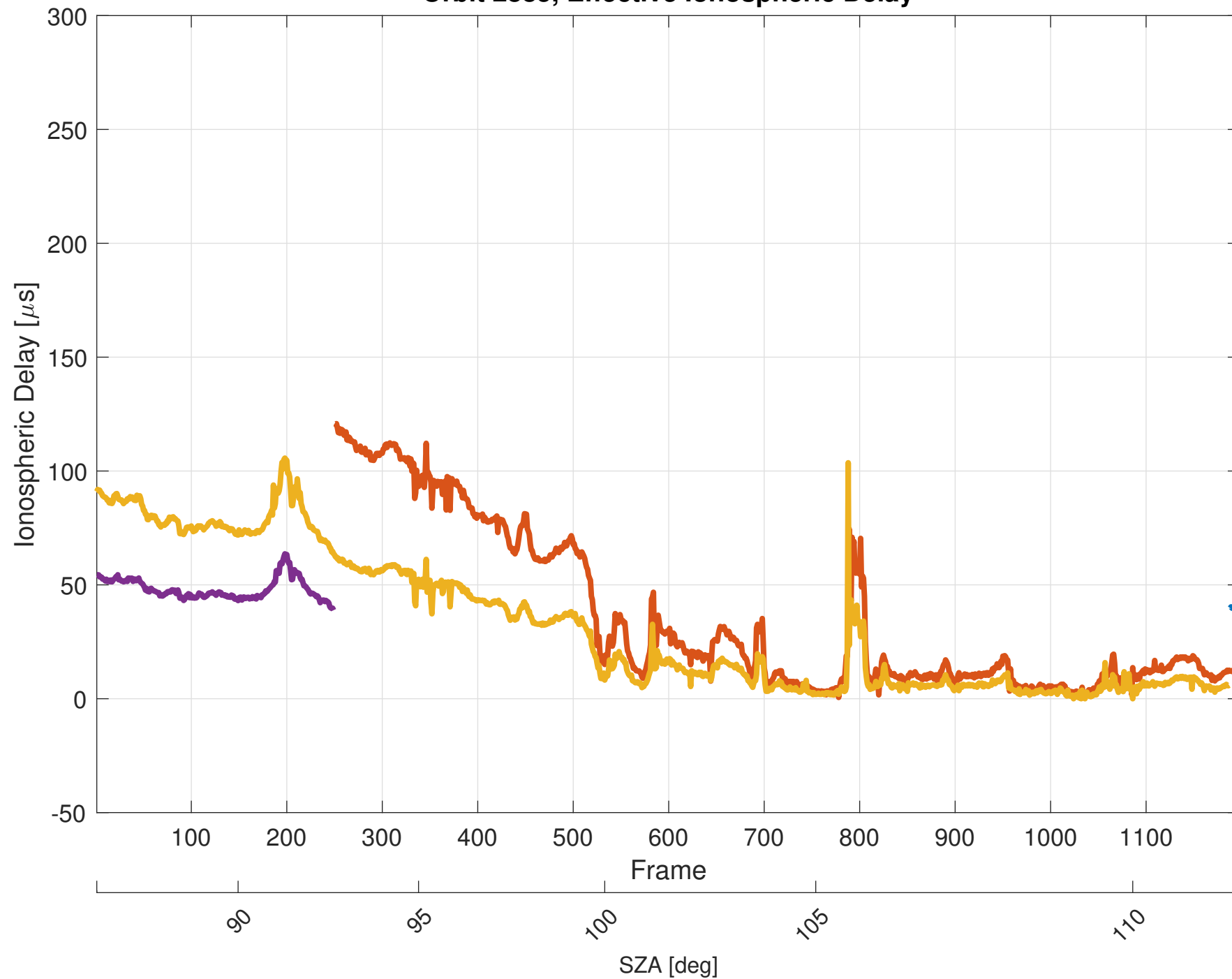
Orbit 2885, Effective Ionospheric Delay
