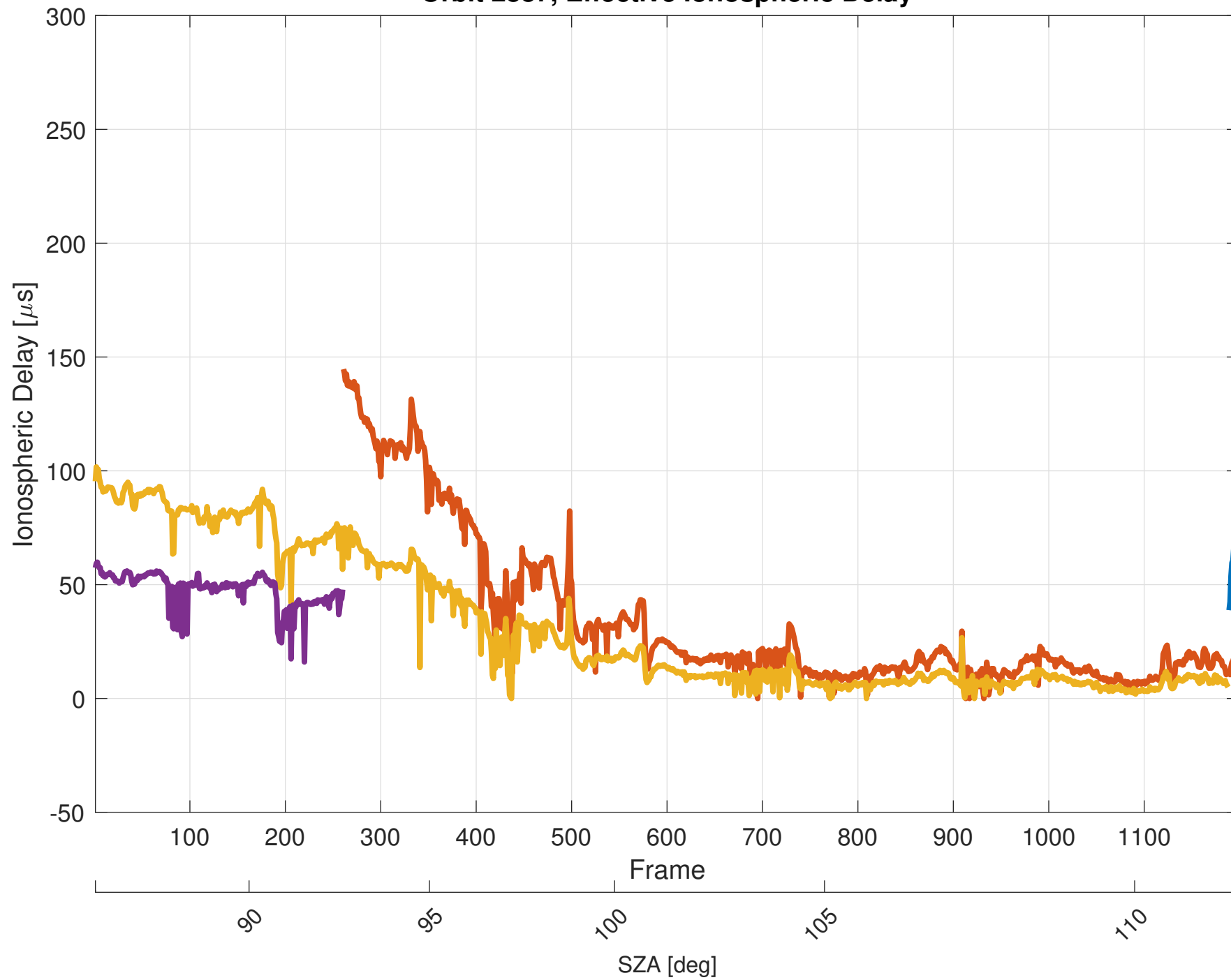
Orbit 2887, Effective Ionospheric Delay
