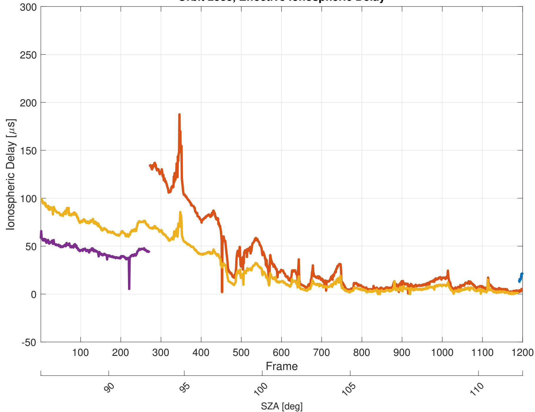
Orbit 2888, Effective Ionospheric Delay
