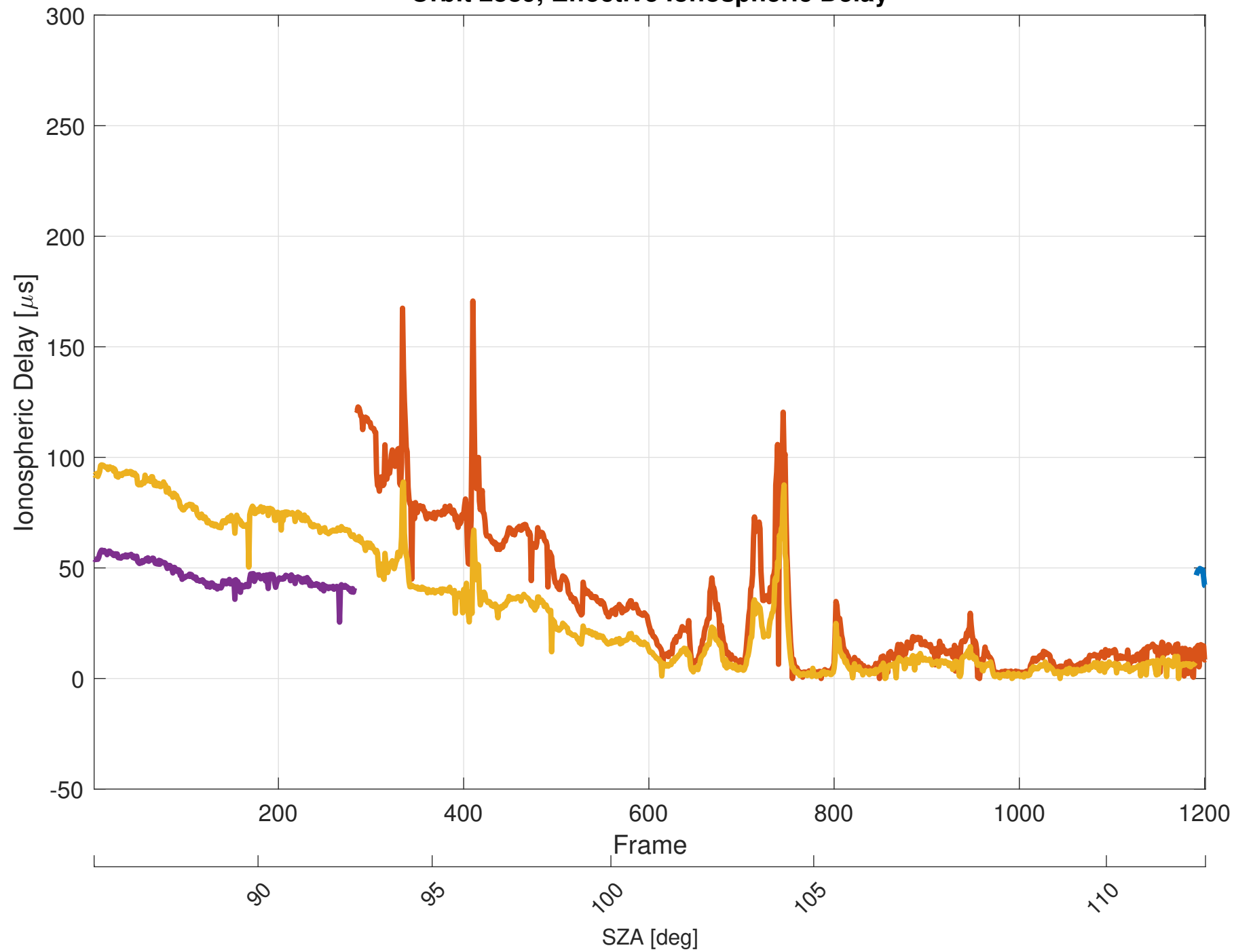
Orbit 2889, Effective Ionospheric Delay
