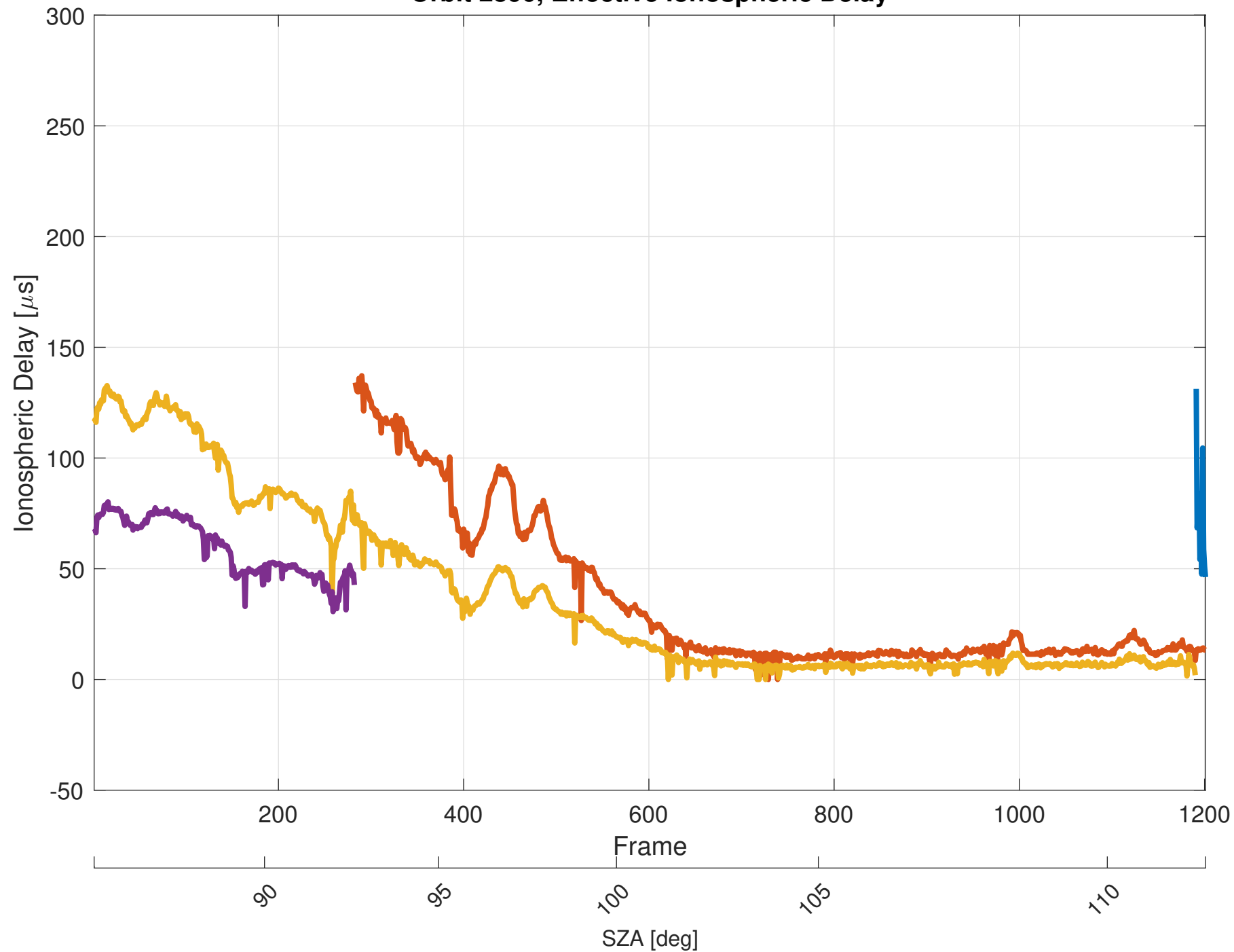
Orbit 2890, Effective Ionospheric Delay
