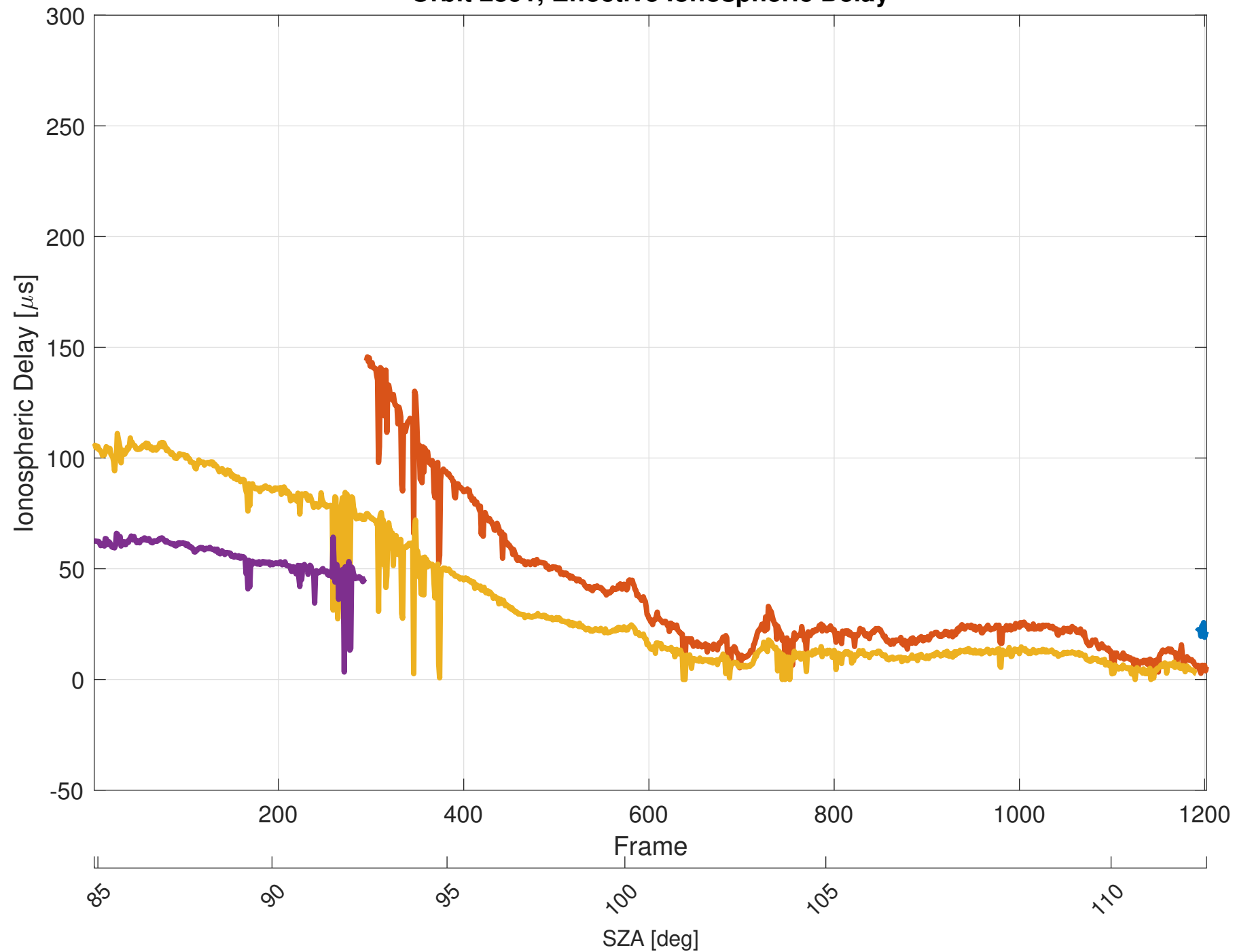
Orbit 2891, Effective Ionospheric Delay
