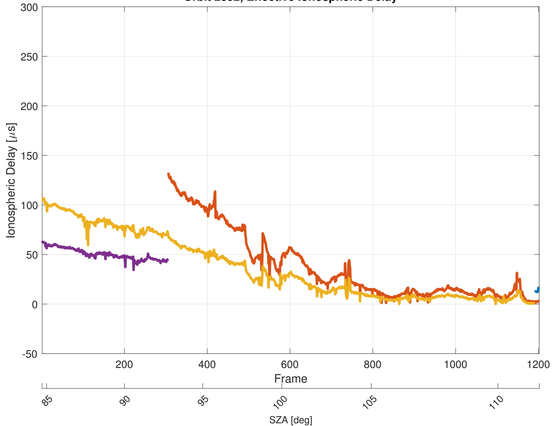
Orbit 2892, Effective Ionospheric Delay
