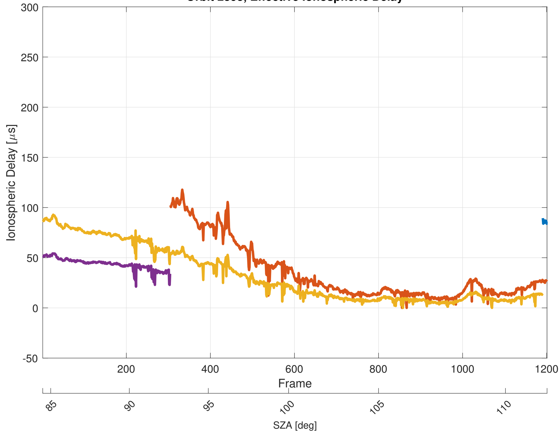
Orbit 2893, Effective Ionospheric Delay
