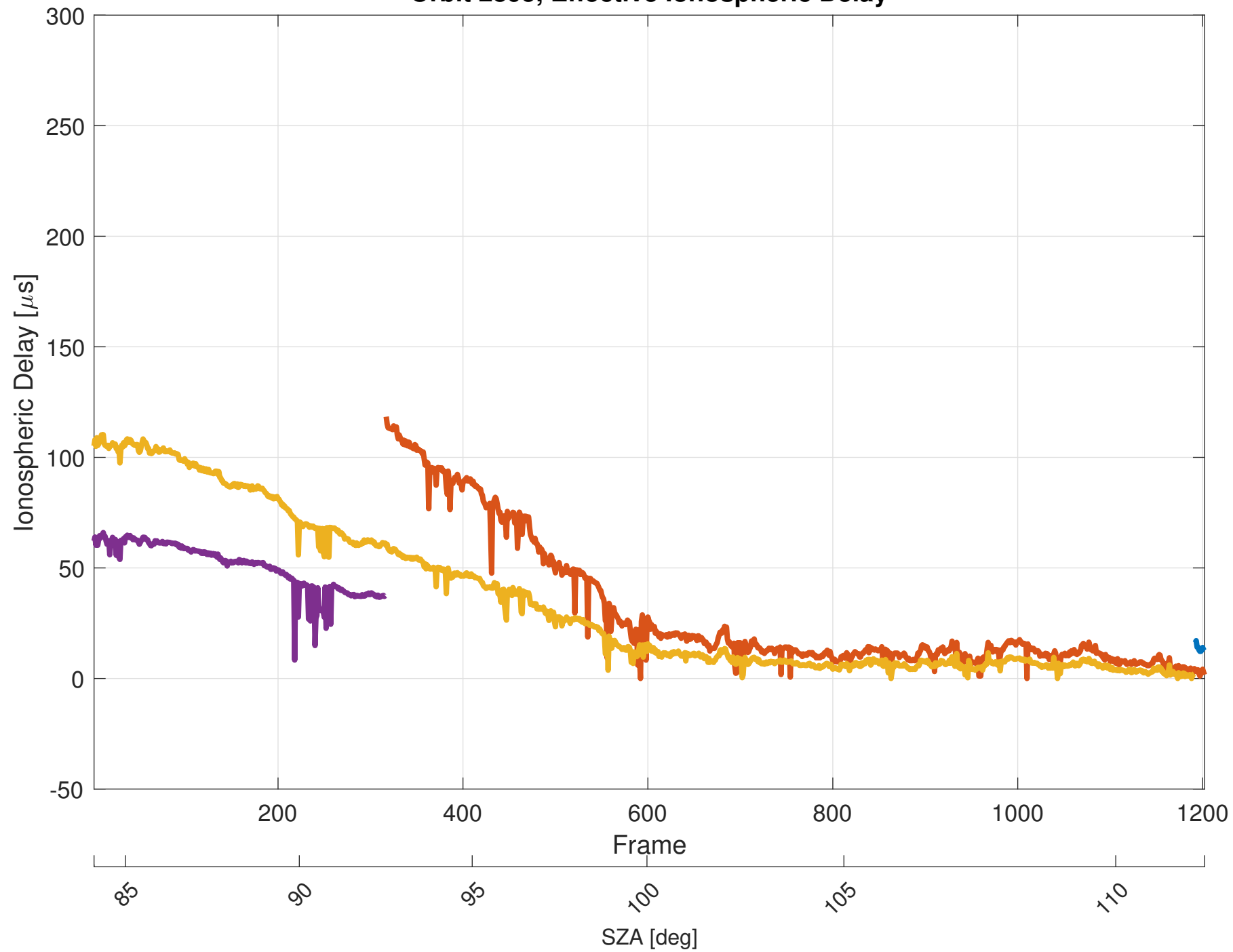
Orbit 2895, Effective Ionospheric Delay
