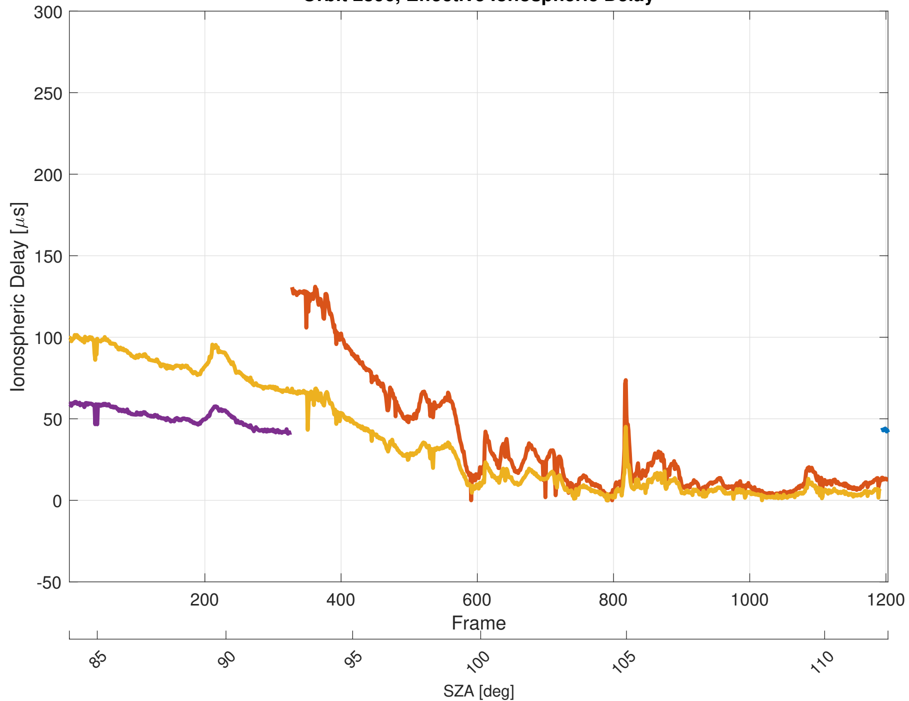
Orbit 2896, Effective Ionospheric Delay
