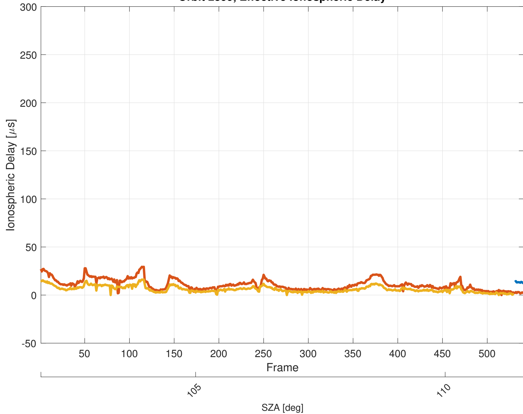
Orbit 2899, Effective Ionospheric Delay
