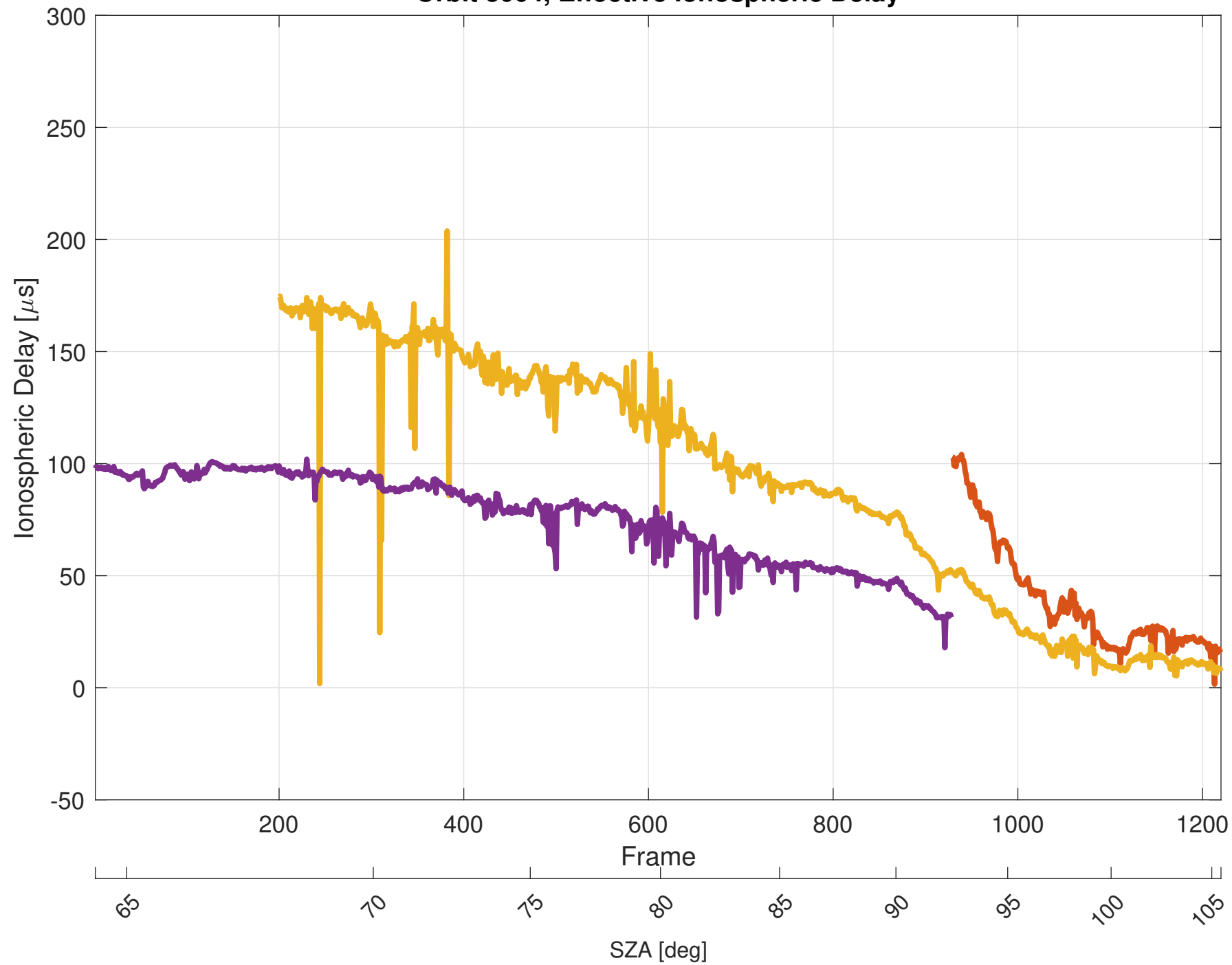
Orbit 3004, Effective Ionospheric Delay
