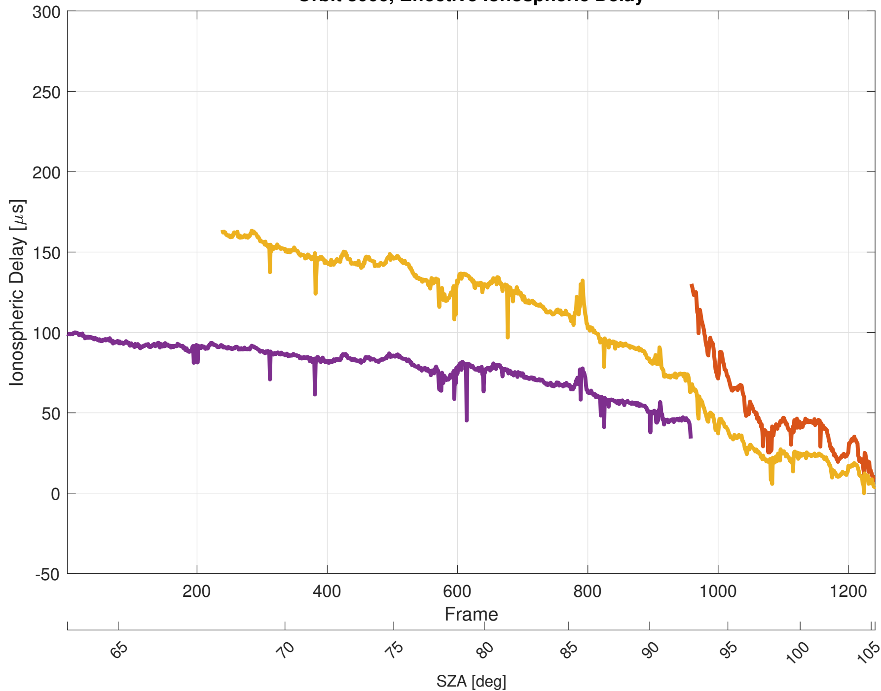
Orbit 3006, Effective Ionospheric Delay
