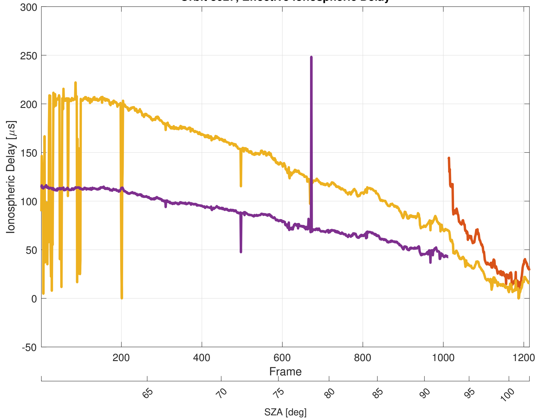
Orbit 3027, Effective Ionospheric Delay
