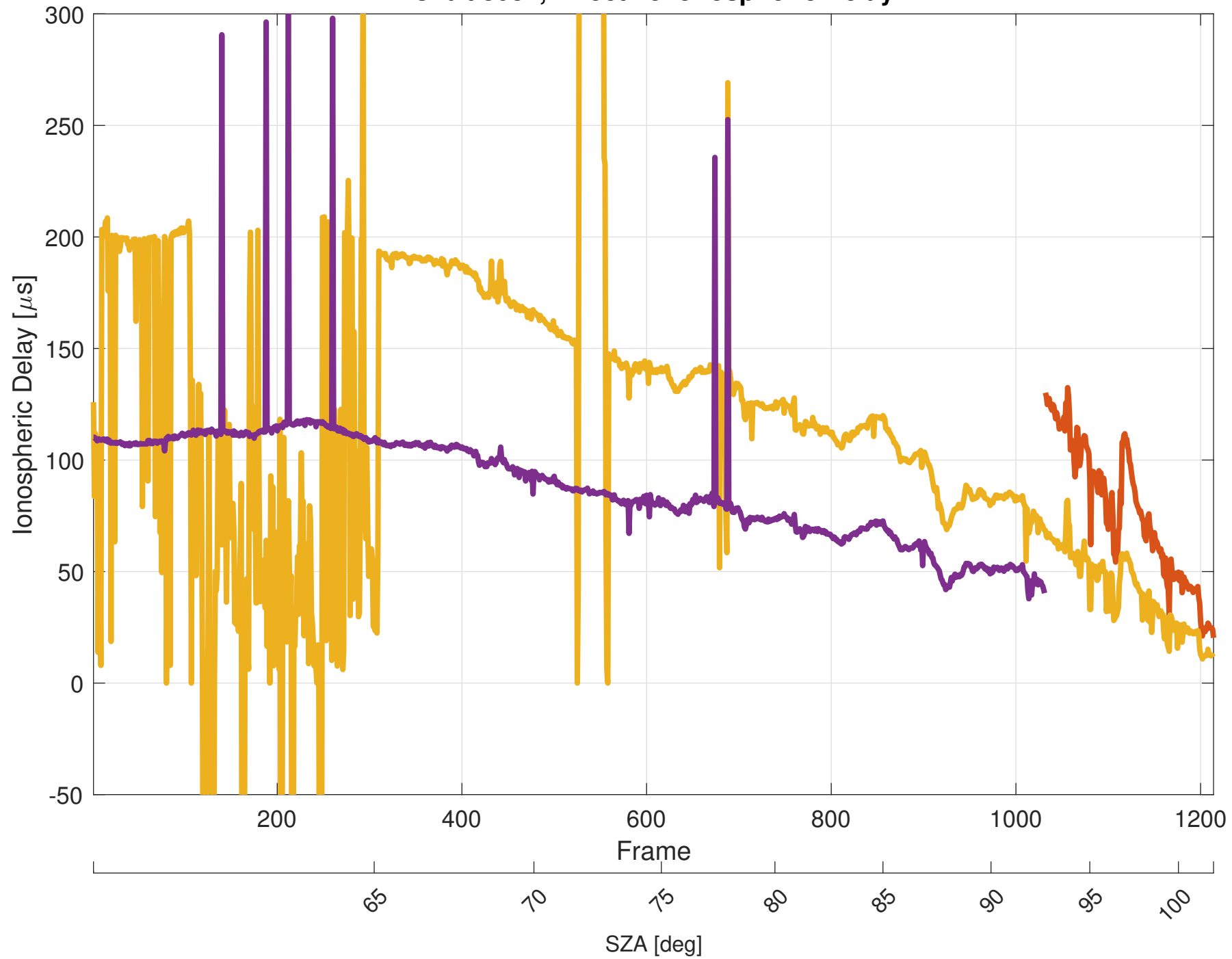
Orbit 3032, Effective Ionospheric Delay
