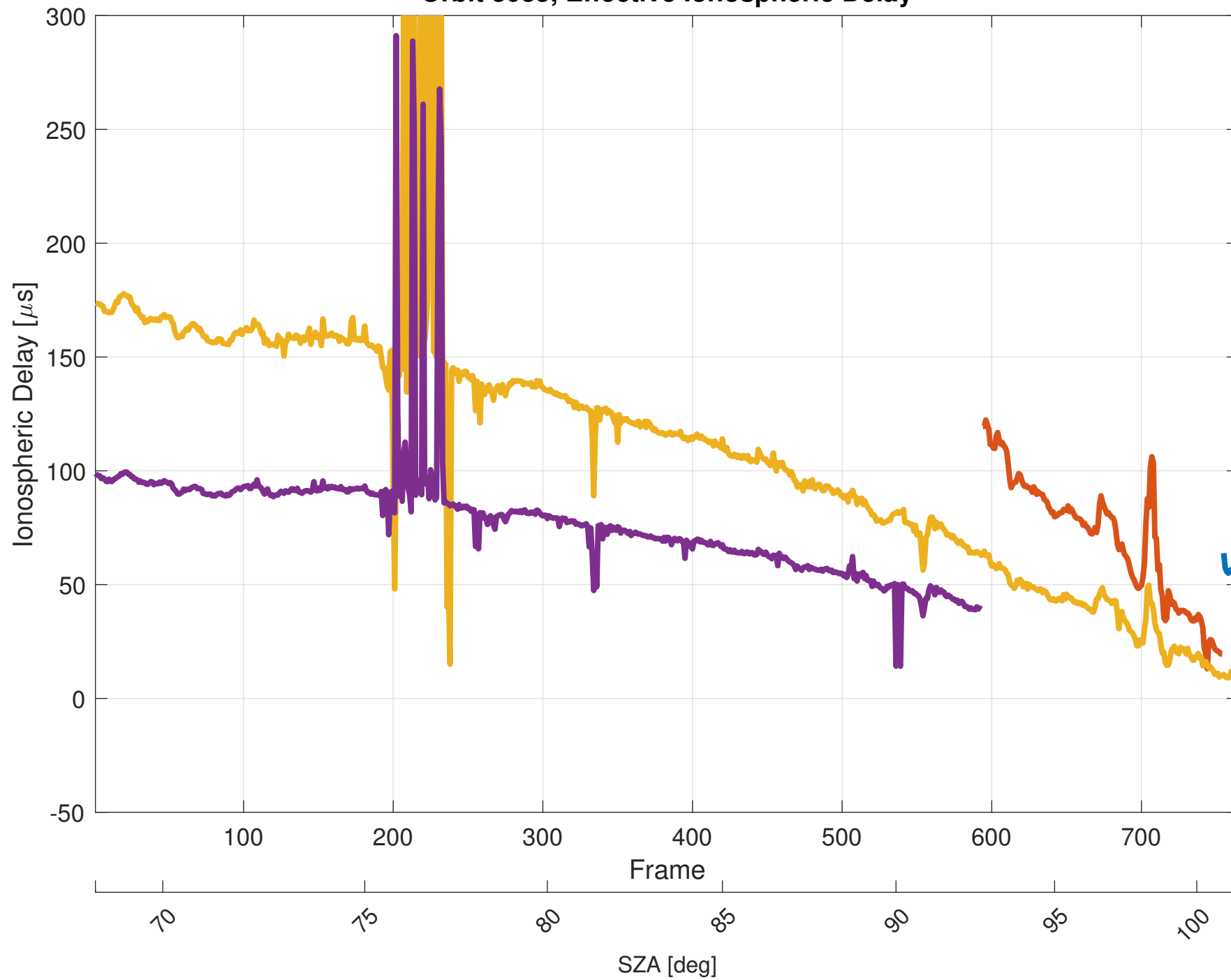
Orbit 3035, Effective Ionospheric Delay
