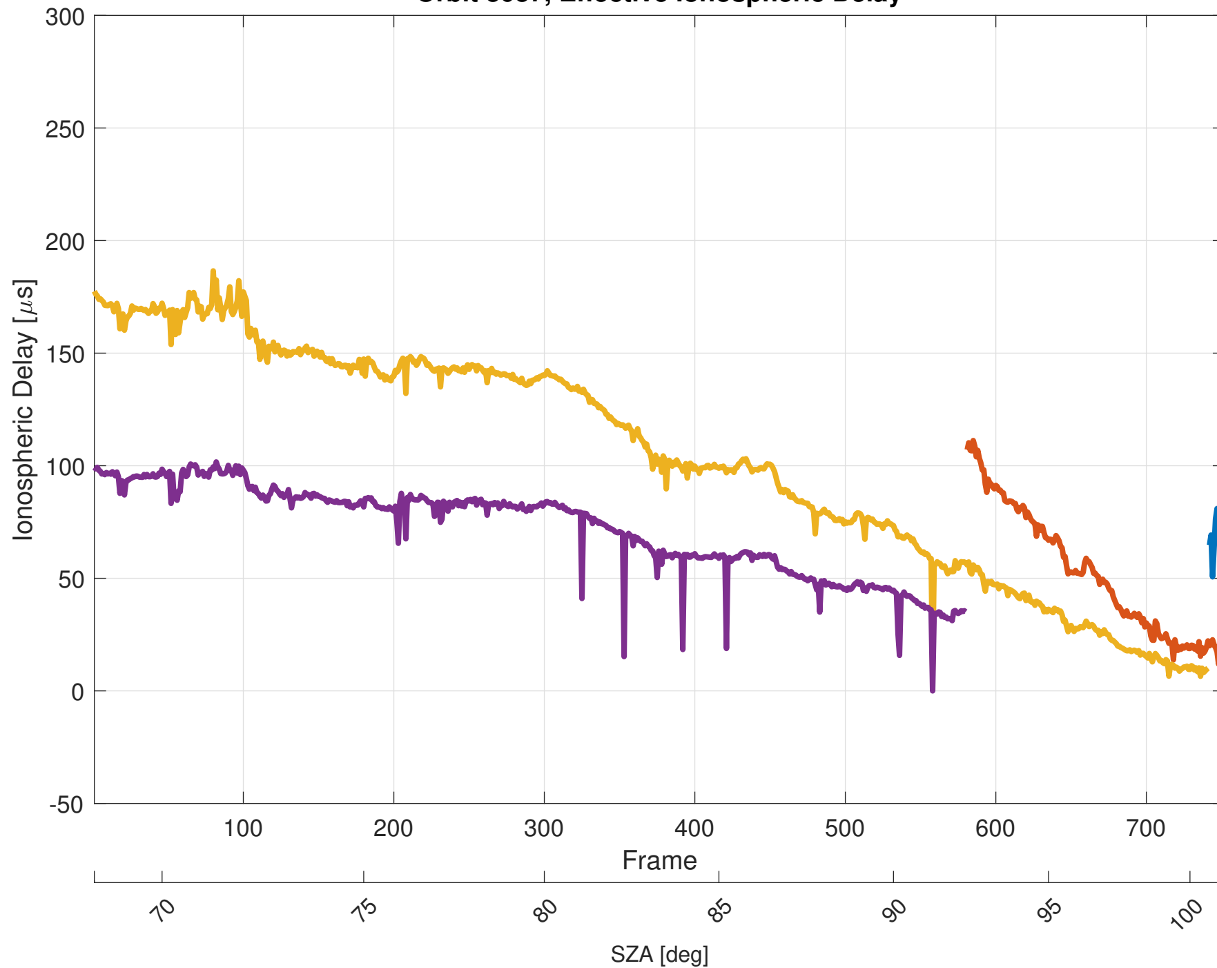
Orbit 3037, Effective Ionospheric Delay
