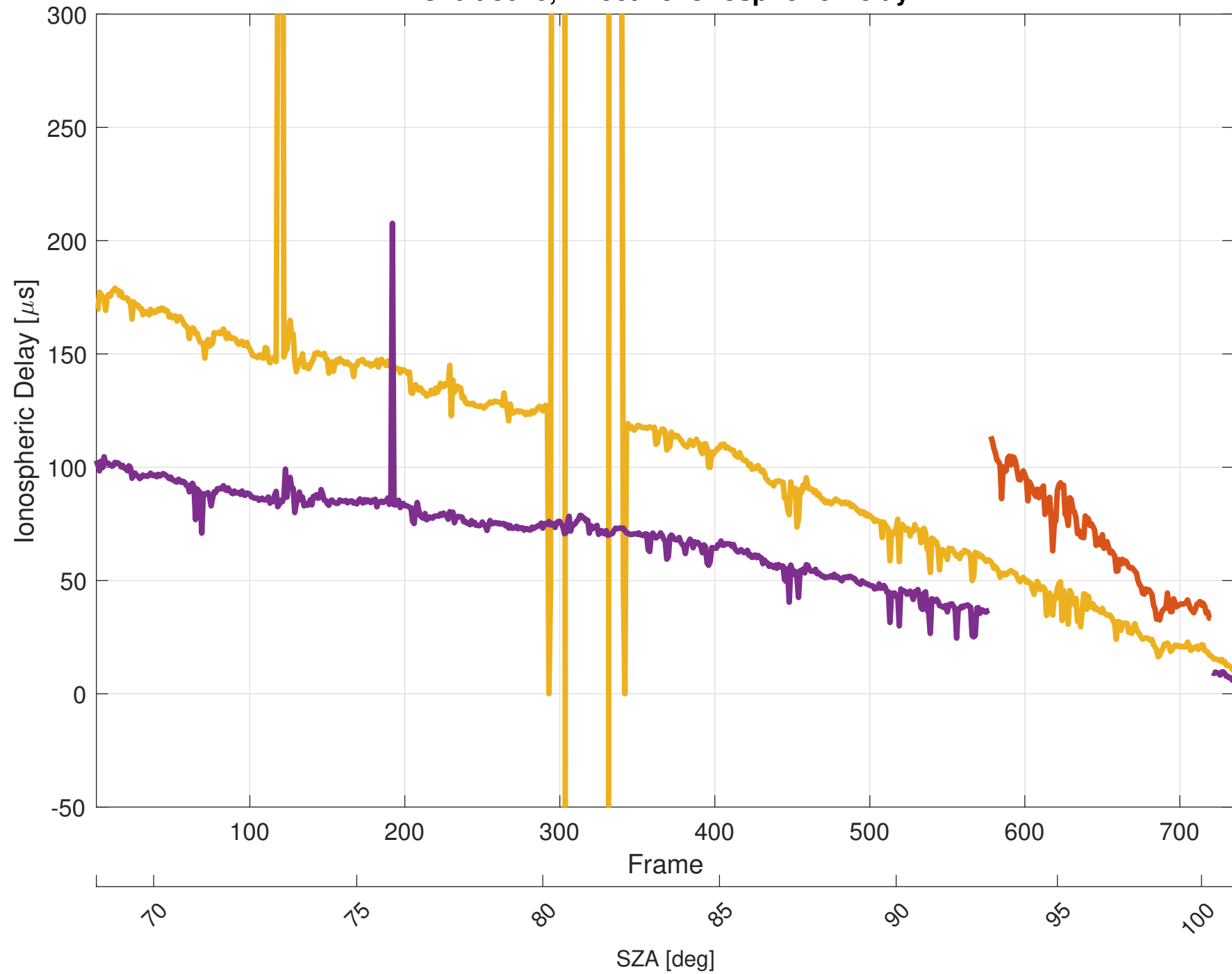
Orbit 3040, Effective Ionospheric Delay
