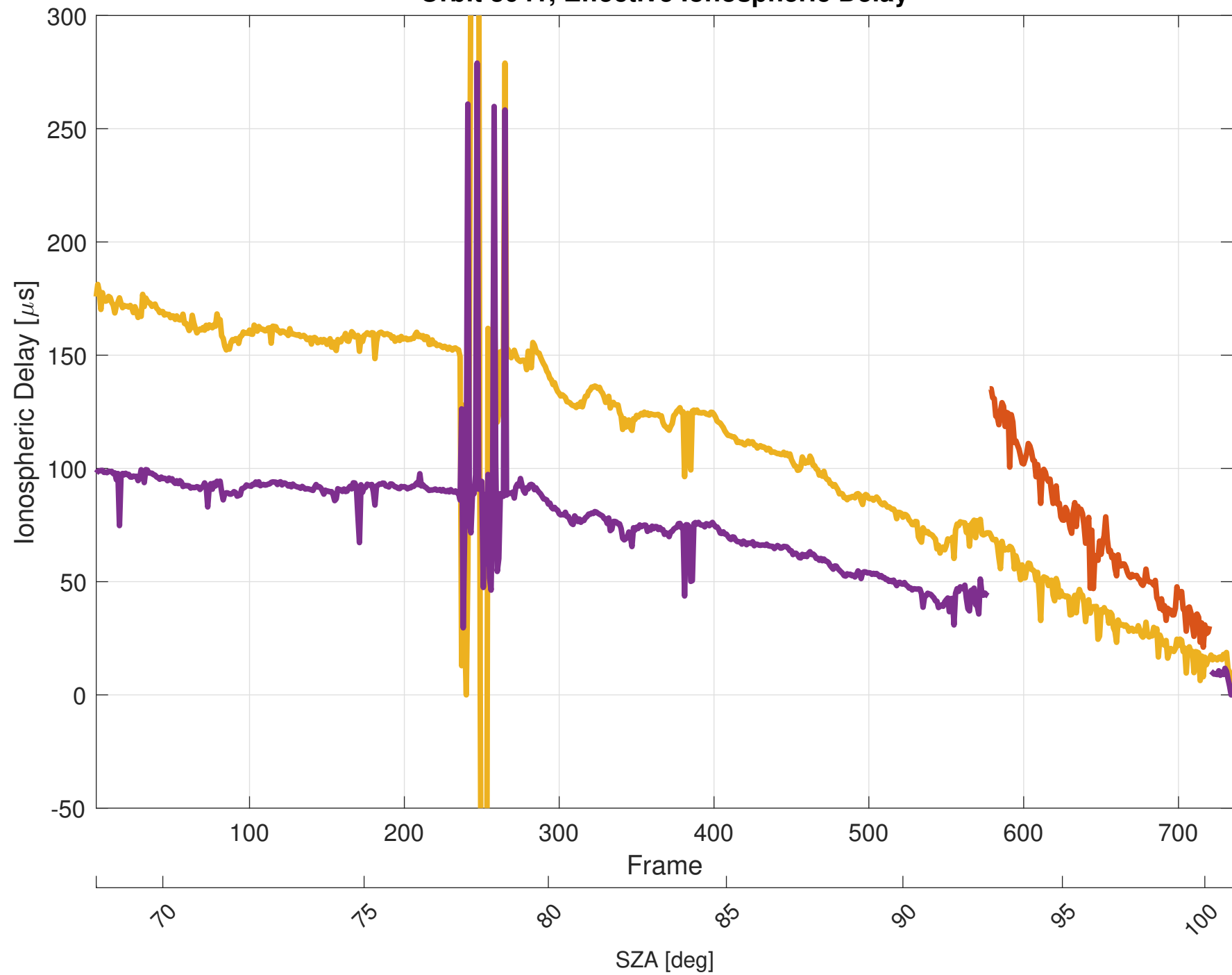
Orbit 3041, Effective Ionospheric Delay
