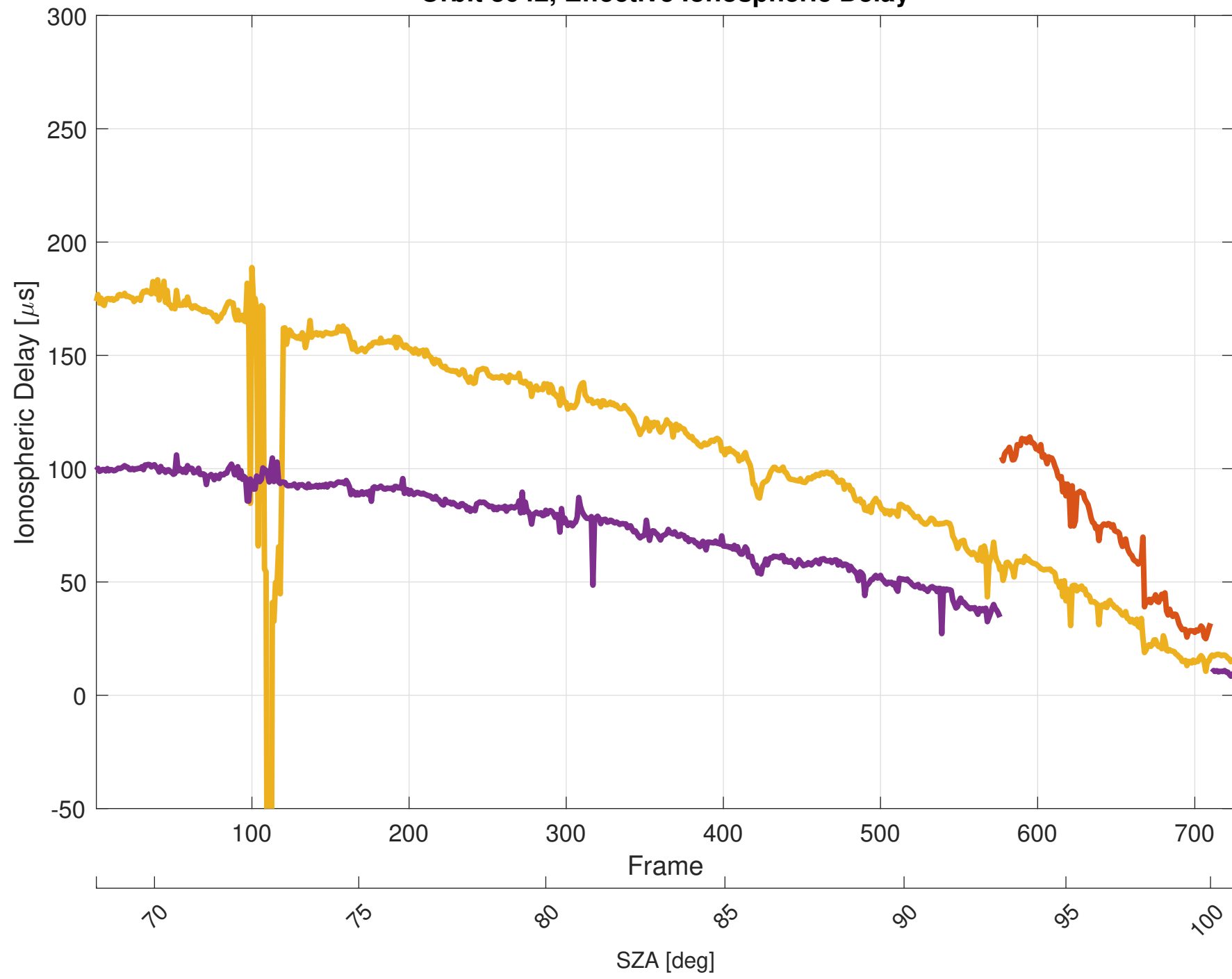
Orbit 3042, Effective Ionospheric Delay
