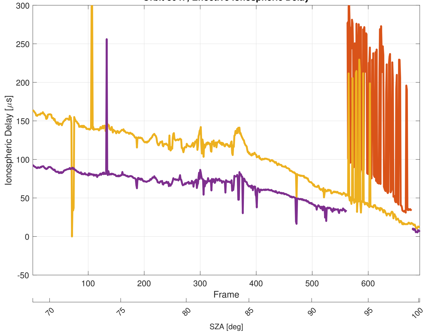
Orbit 3047, Effective Ionospheric Delay
