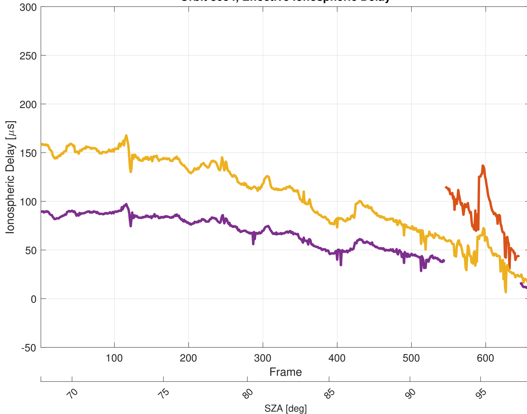
Orbit 3054, Effective Ionospheric Delay
