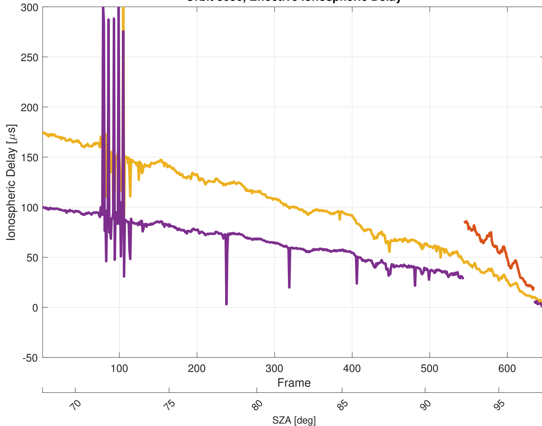
Orbit 3056, Effective Ionospheric Delay
