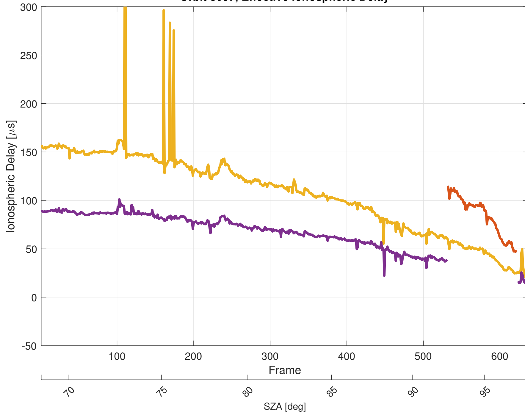
Orbit 3057, Effective Ionospheric Delay
