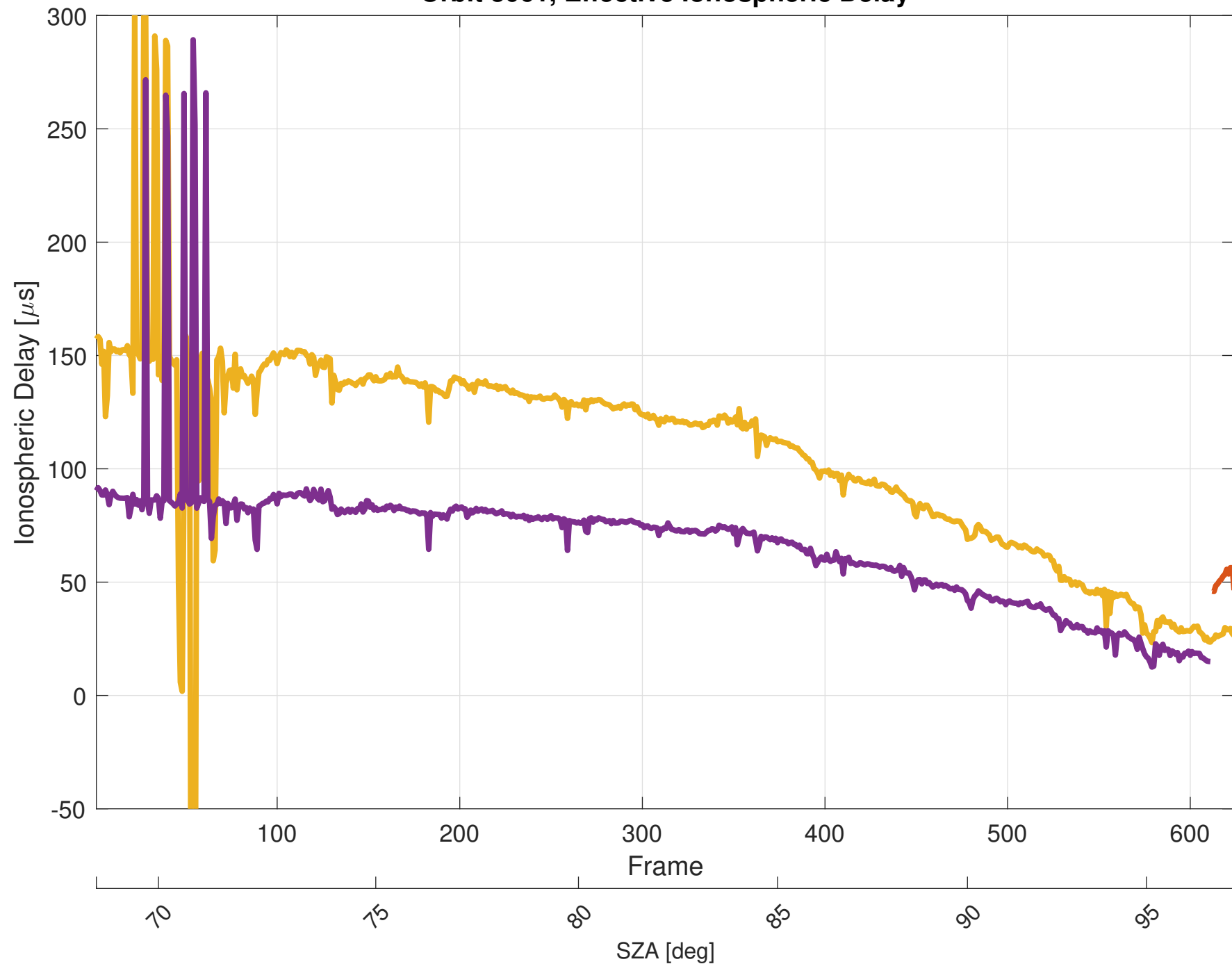
Orbit 3061, Effective Ionospheric Delay
