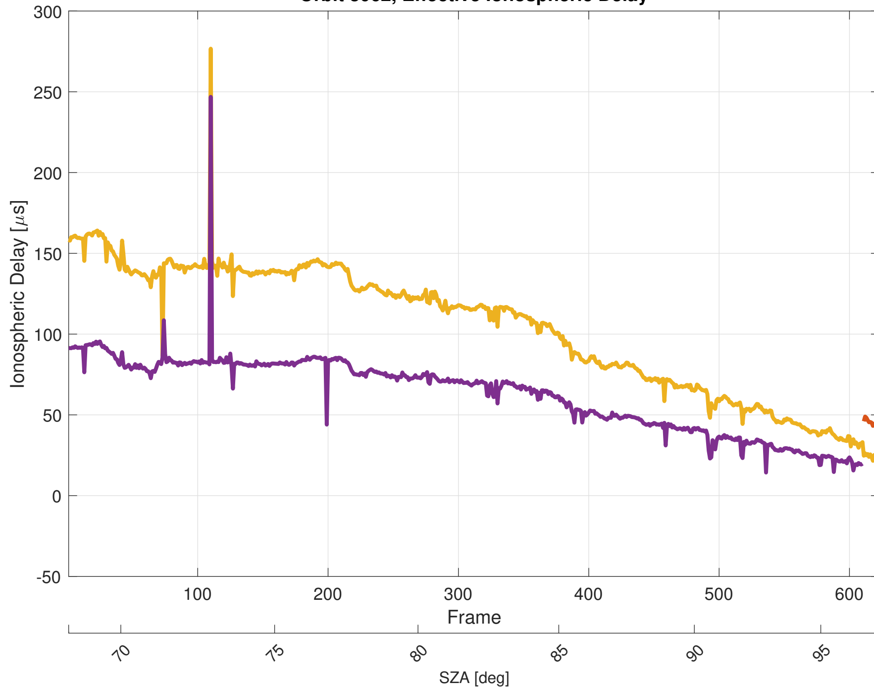
Orbit 3062, Effective Ionospheric Delay
