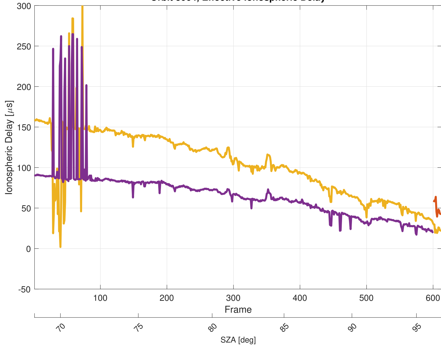
Orbit 3064, Effective Ionospheric Delay
