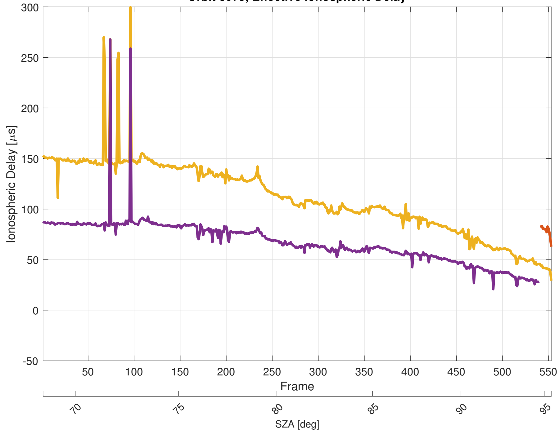
Orbit 3075, Effective Ionospheric Delay
