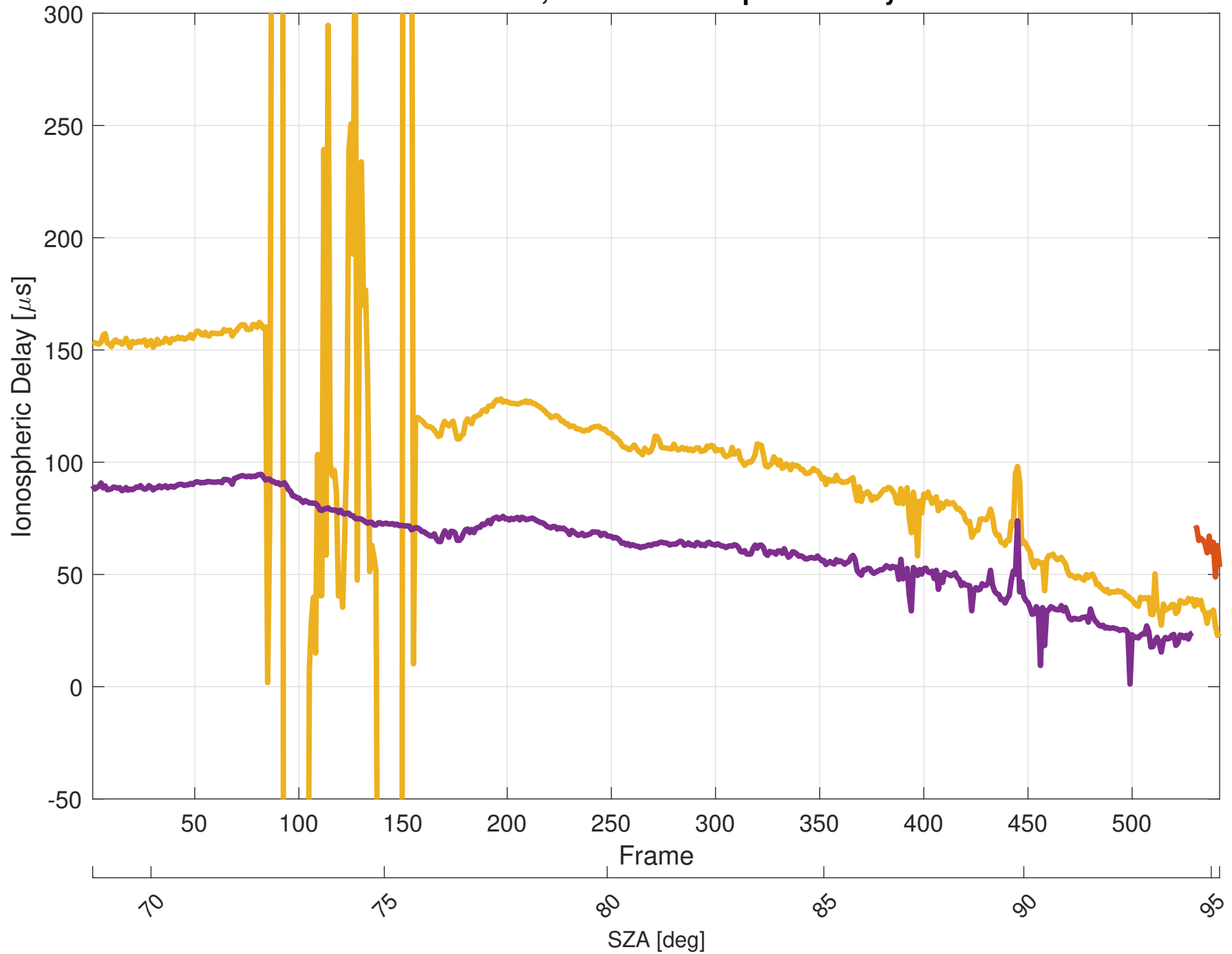
Orbit 3076, Effective Ionospheric Delay
