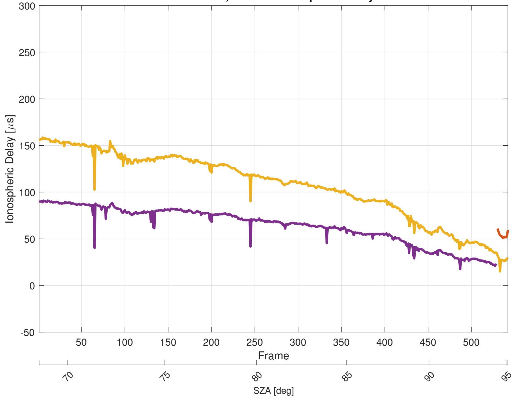
Orbit 3077, Effective Ionospheric Delay
