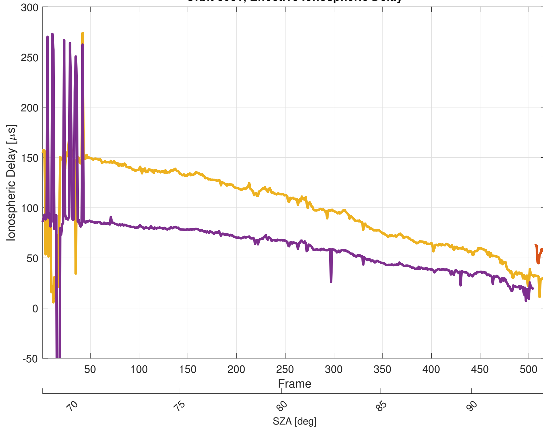
Orbit 3081, Effective Ionospheric Delay
