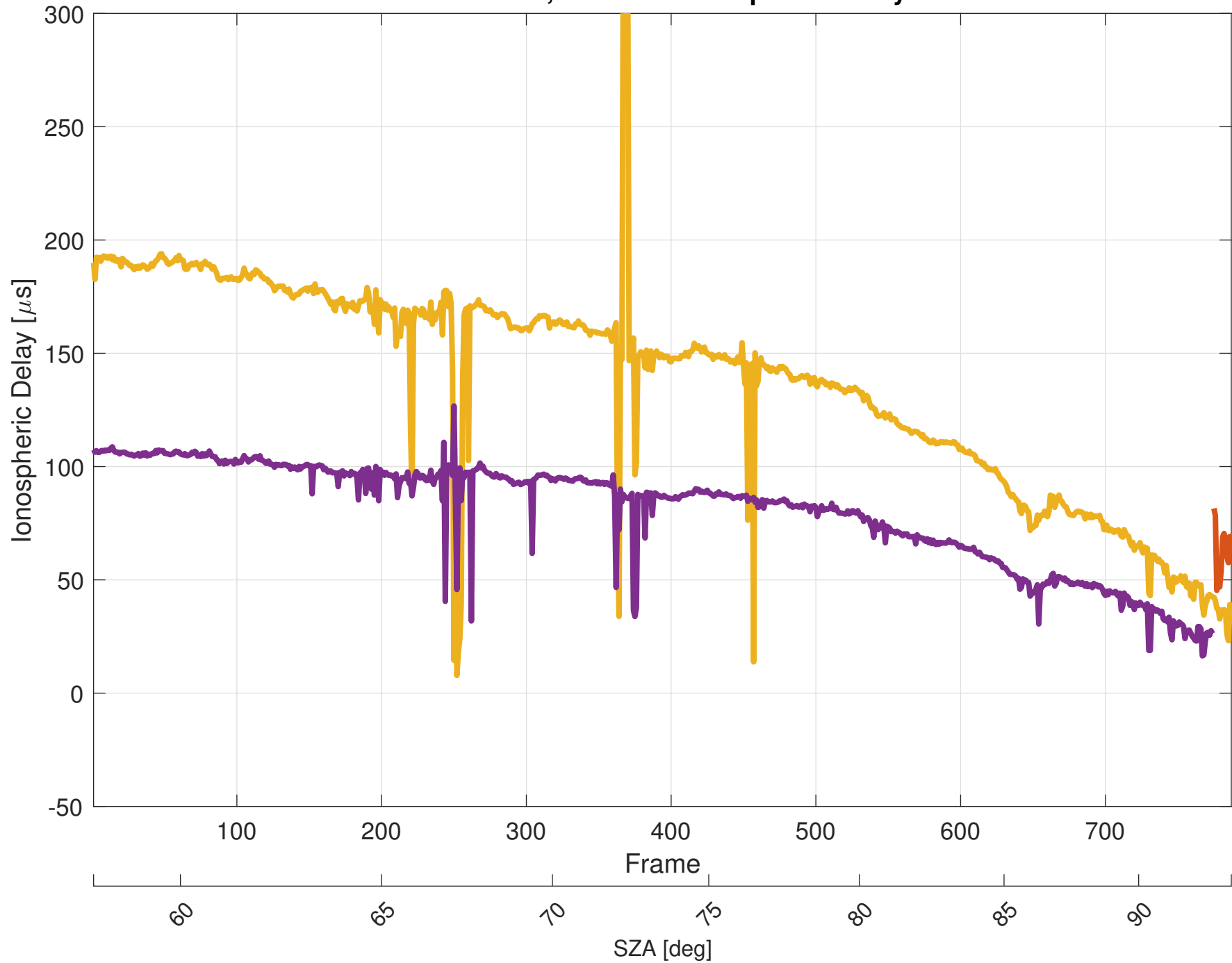
Orbit 3085, Effective Ionospheric Delay
