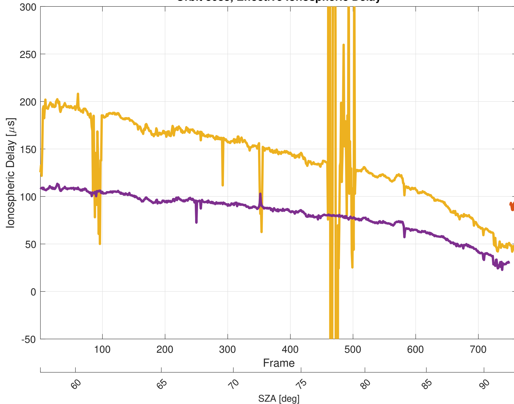
Orbit 3088, Effective Ionospheric Delay
