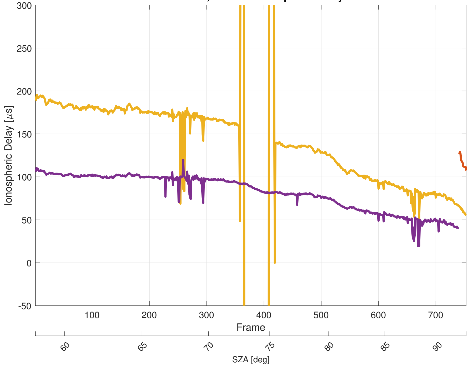
Orbit 3089, Effective Ionospheric Delay
