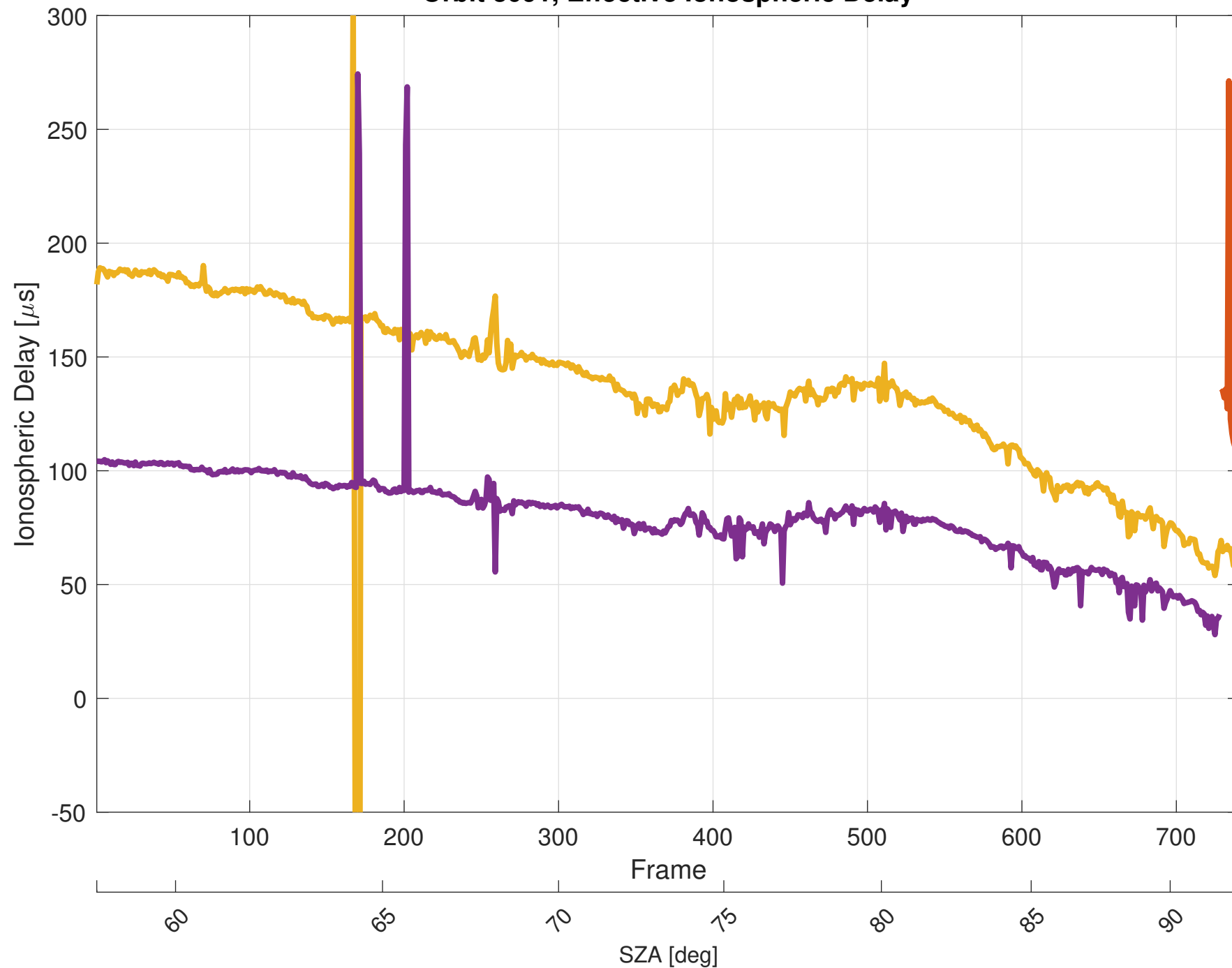
Orbit 3091, Effective Ionospheric Delay
