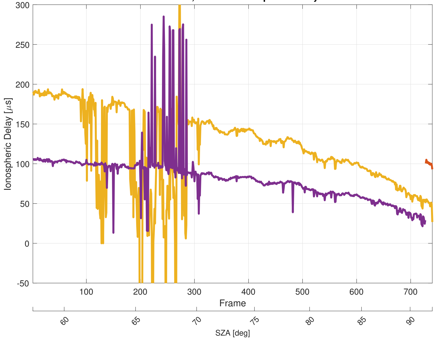
Orbit 3092, Effective Ionospheric Delay
